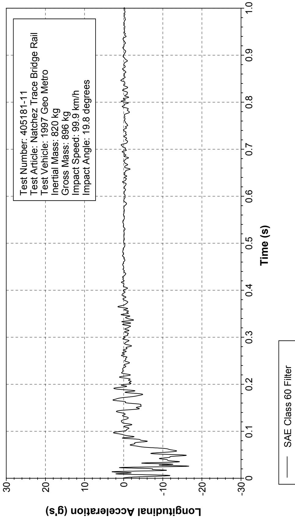
Figure 315. Vehicle longitudinal accelerometer trace for test 405181-11 (accelerometer located at center of gravity).
