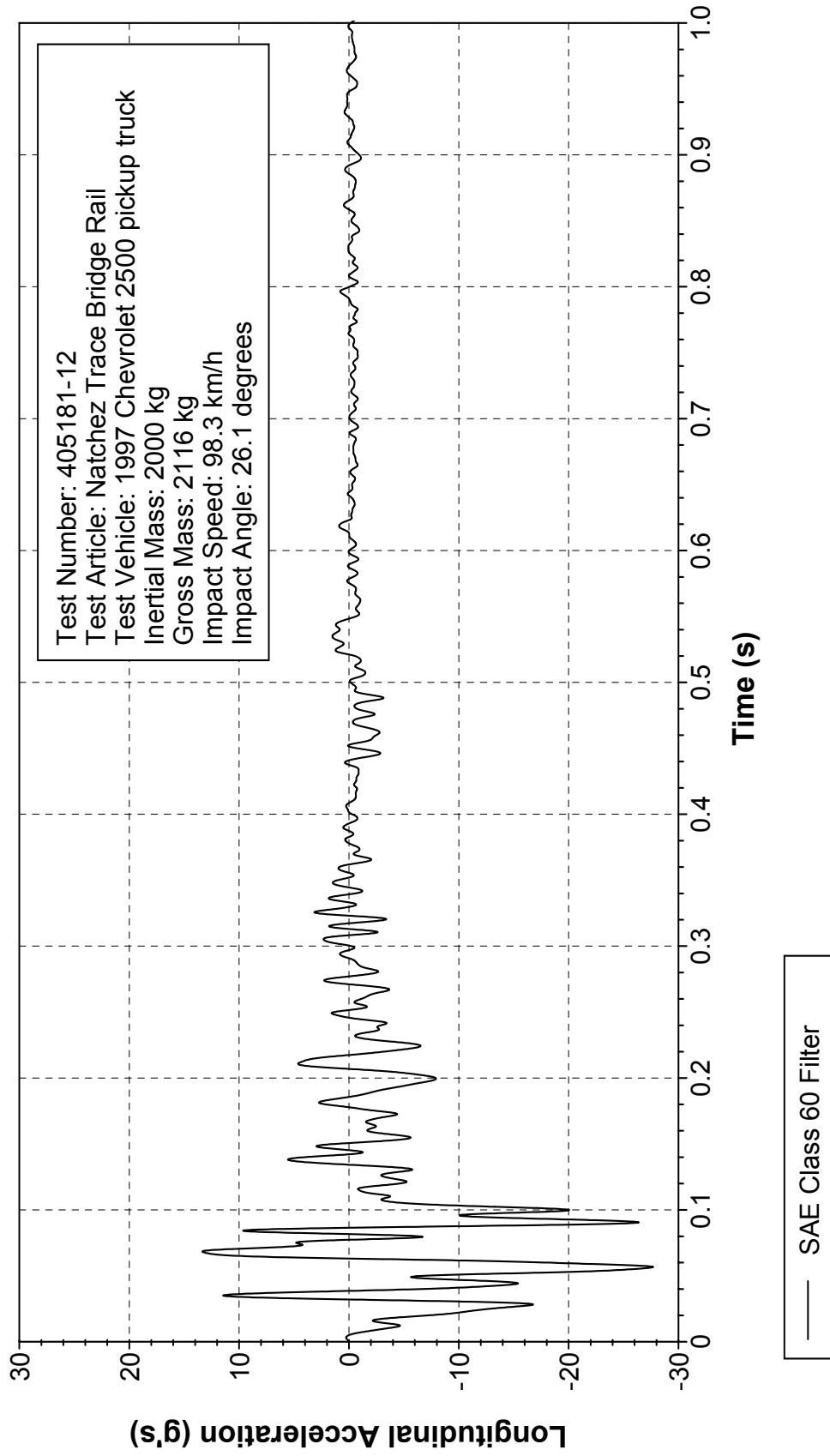
Figure 322. Vehicle longitudinal accelerometer trace for test 405181-12 (accelerometer located at center of gravity).
