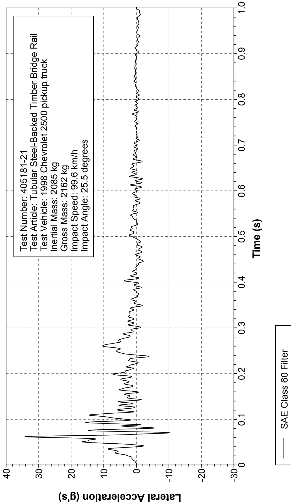
Figure 330. Vehicle lateral accelerometer trace for test 405181-21 (accelerometer located at center of gravity).
