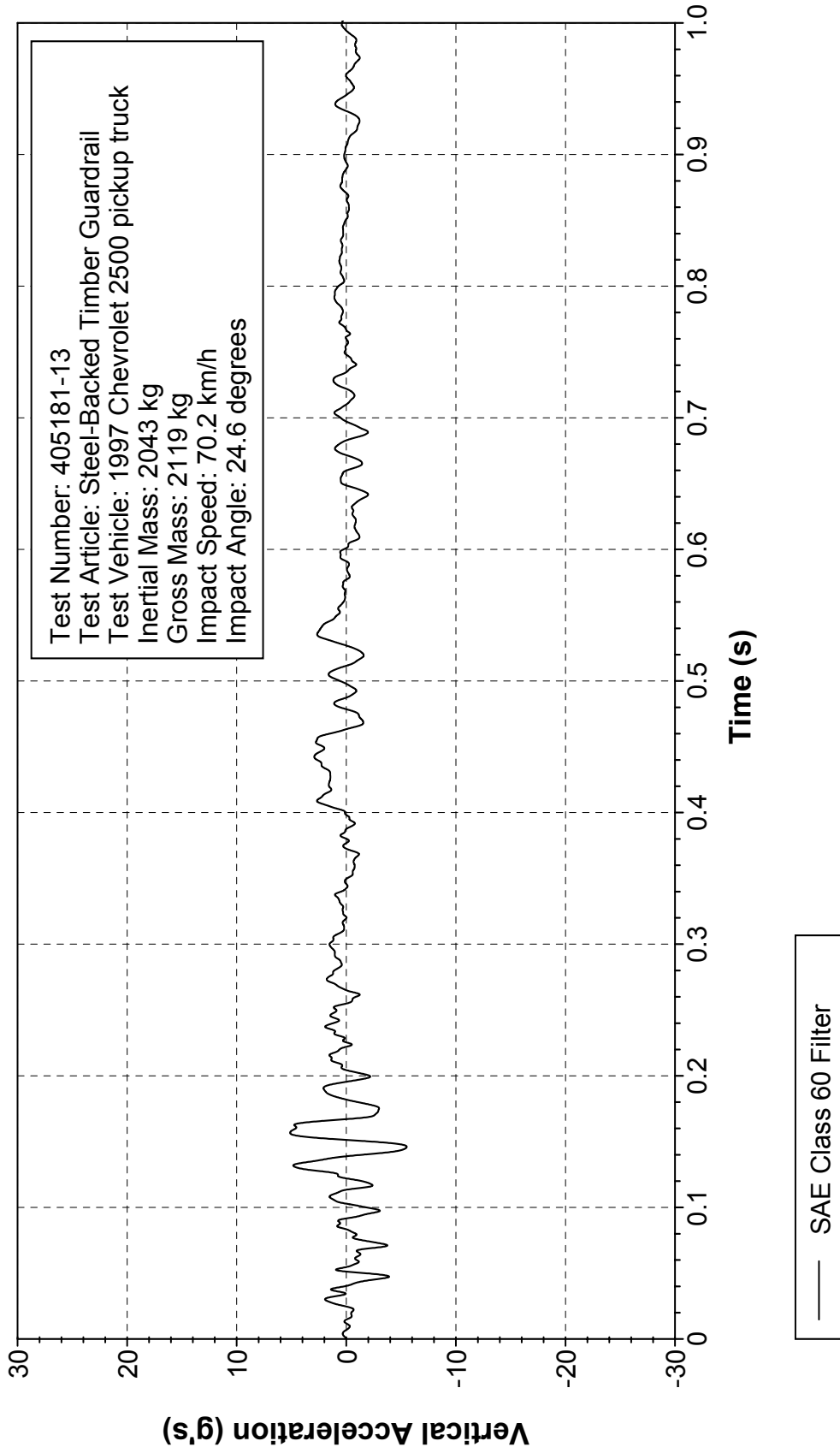
Figure 270. Vehicle vertical accelerometer trace for test 405181-13 (accelerometer located at center of gravity).
