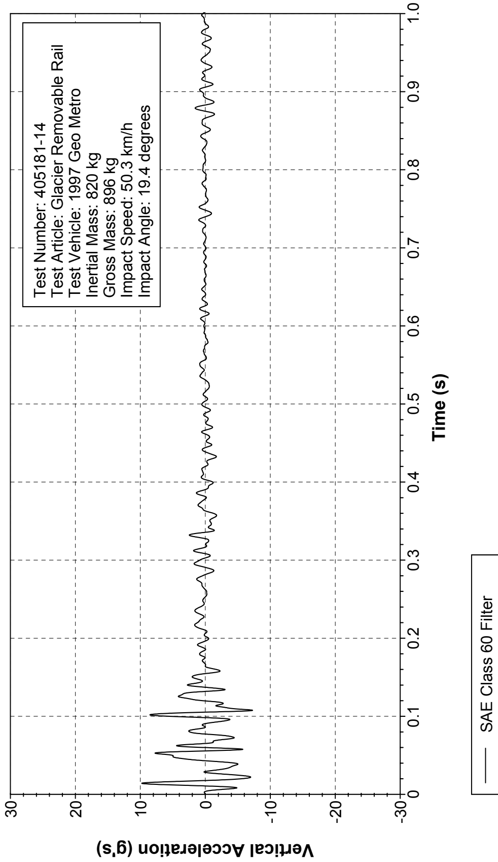
Figure 277. Vehicle vertical accelerometer trace for test 405181-14 (accelerometer located at center of gravity).
