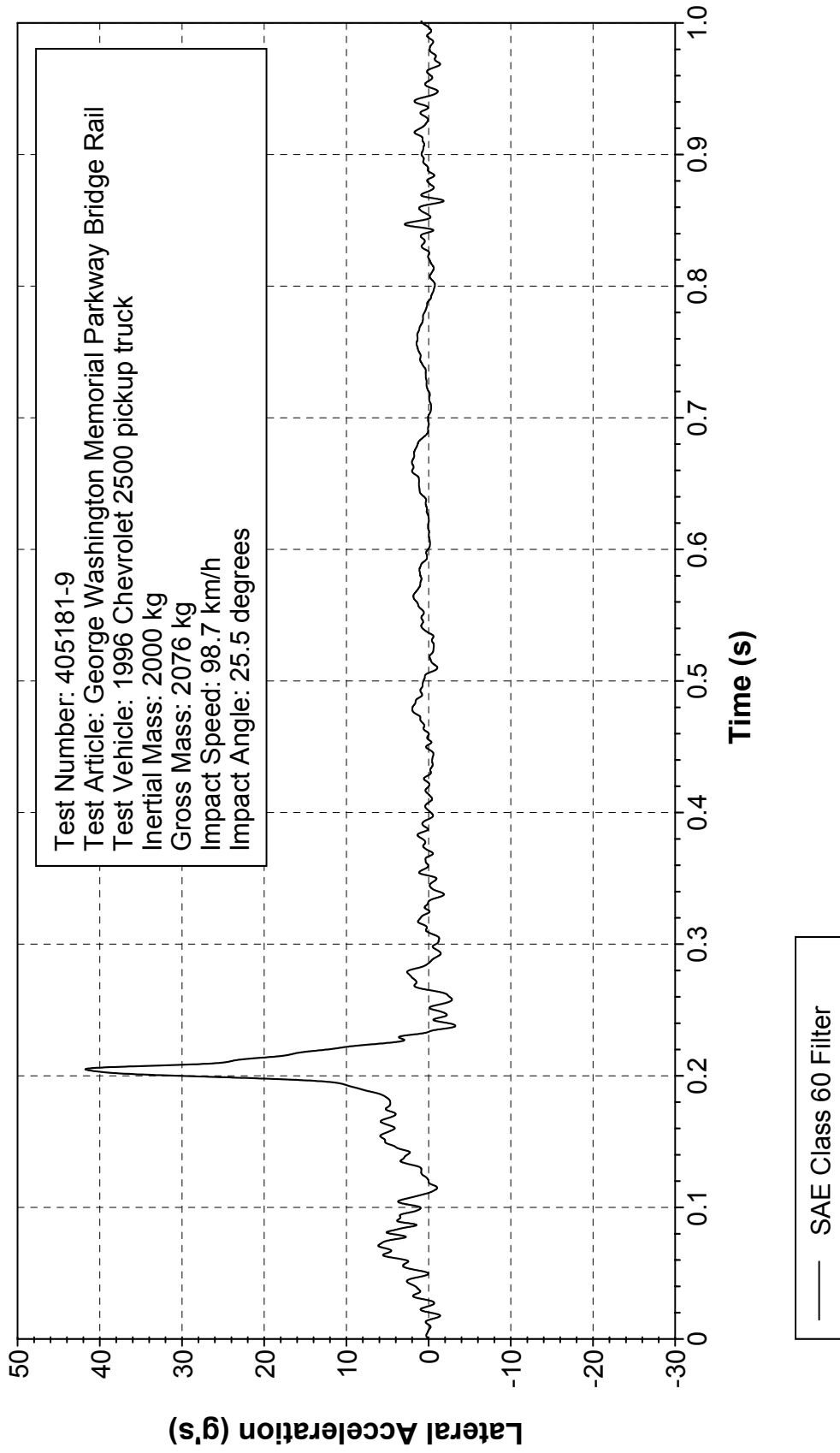
Figure 312. Vehicle lateral accelerometer trace for test 405181-9 (accelerometer located over rear axle).
