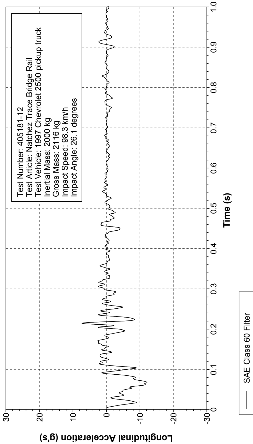
Figure 325. Vehicle longitudinal accelerometer trace for test 405181-12 (accelerometer located over rear axle).
