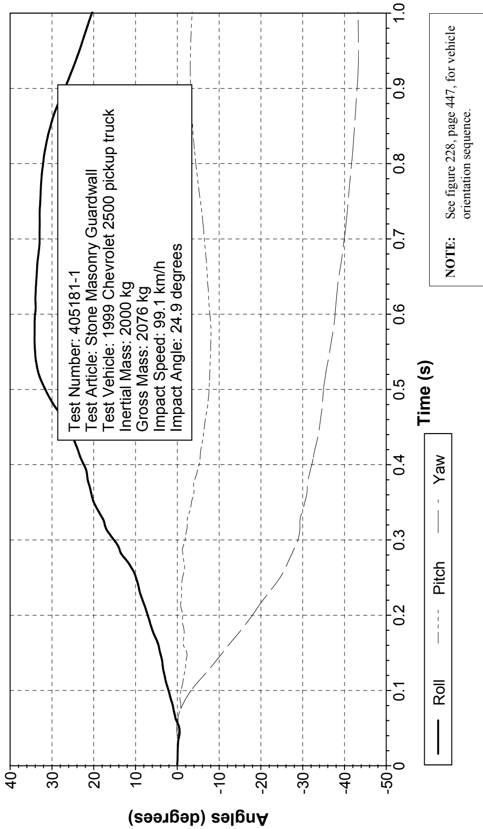
Figure 229. Vehicle angular displacements for test 405181-1.
