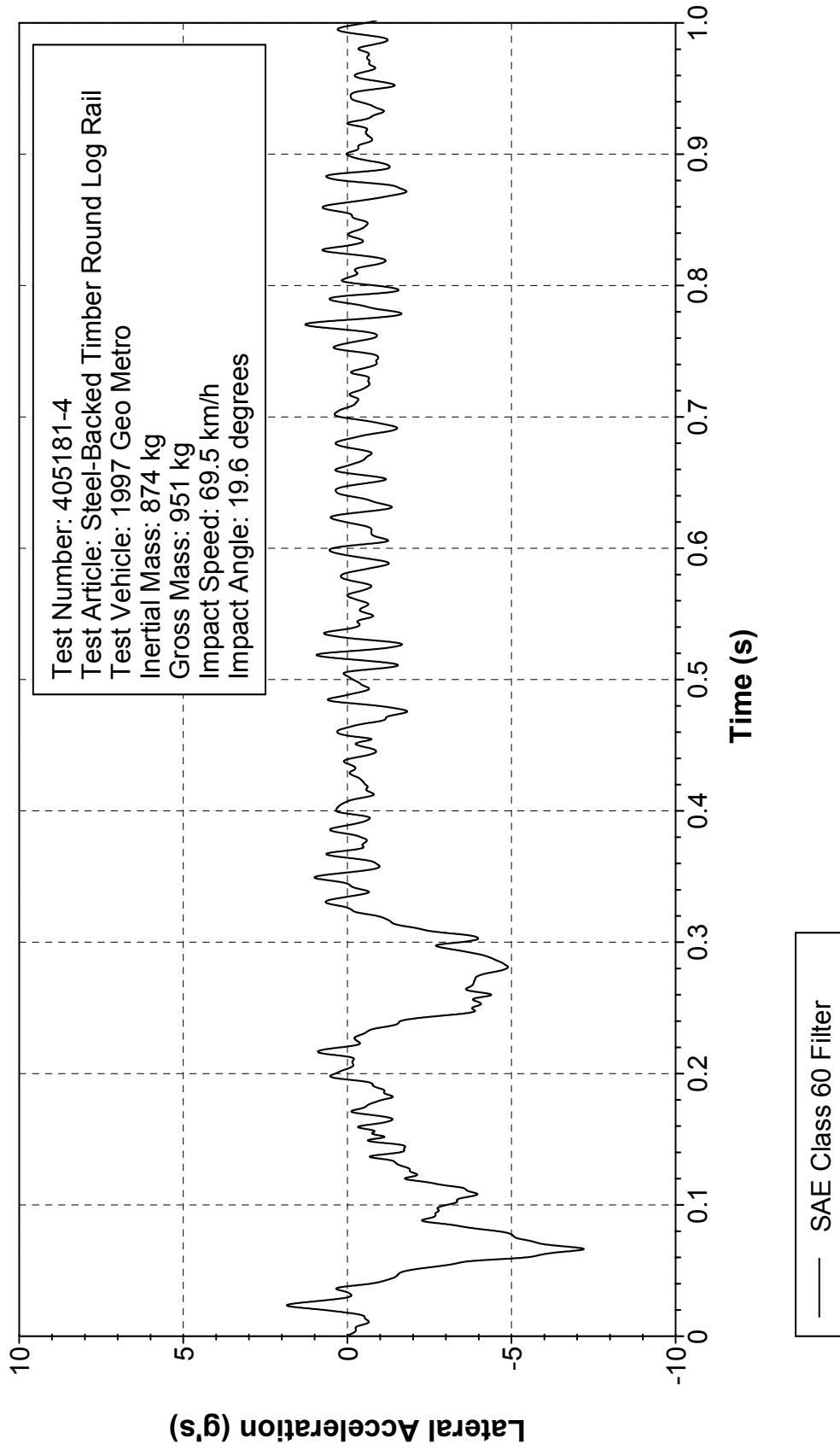
Figure 248. Vehicle lateral accelerometer trace for test 405181-4 (accelerometer located over rear axle).
