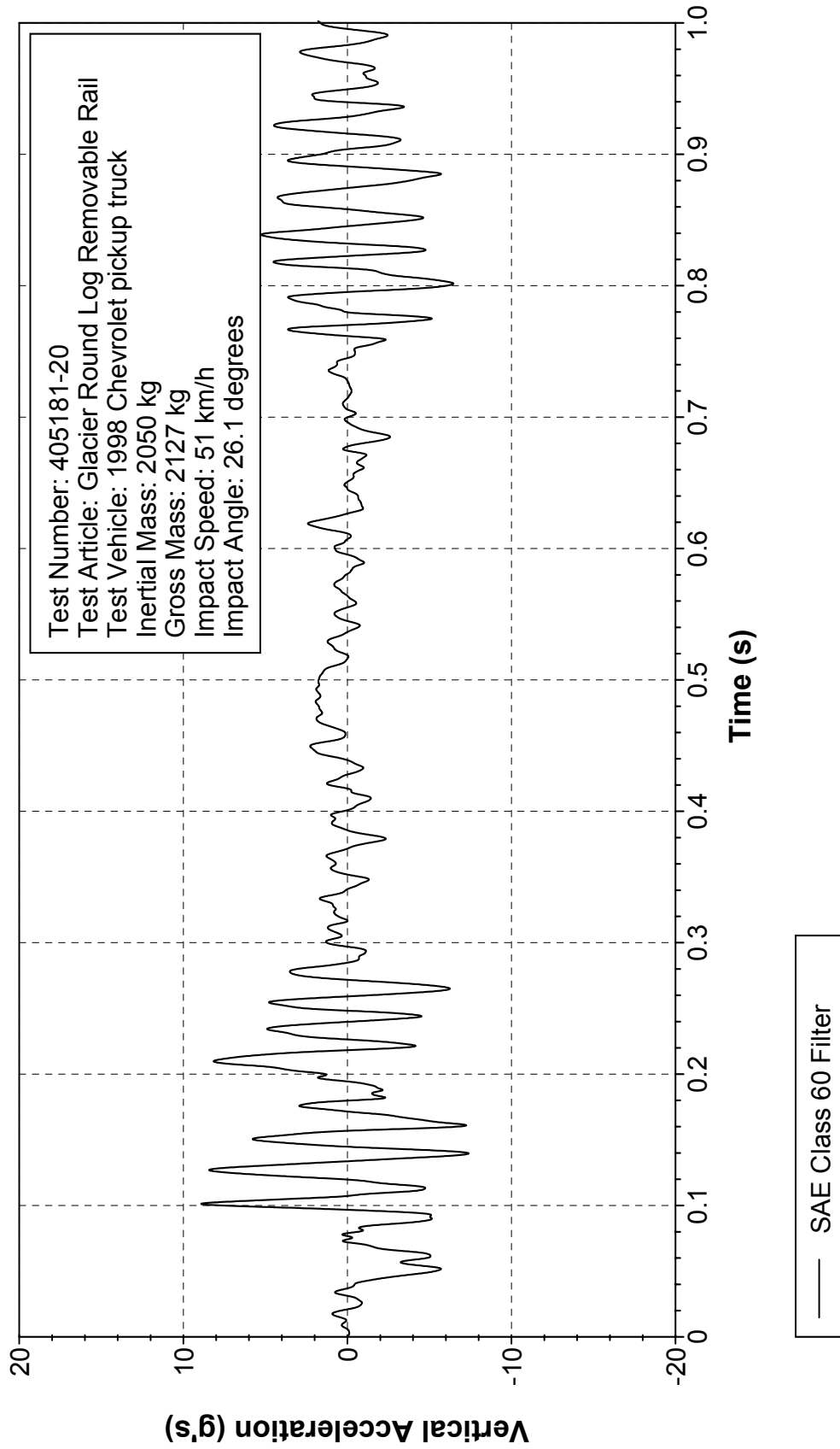
Figure 303. Vehicle vertical accelerometer trace for test 405181-20 (accelerometer located at center of gravity).
