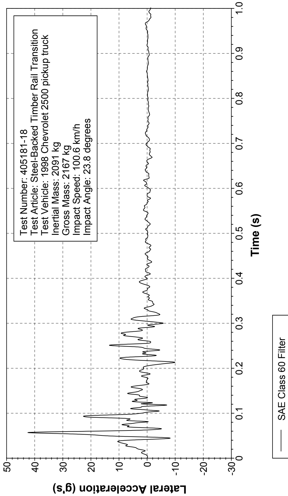
Figure 349. Vehicle lateral accelerometer trace for test 405181-18 (accelerometer located at center of gravity).
