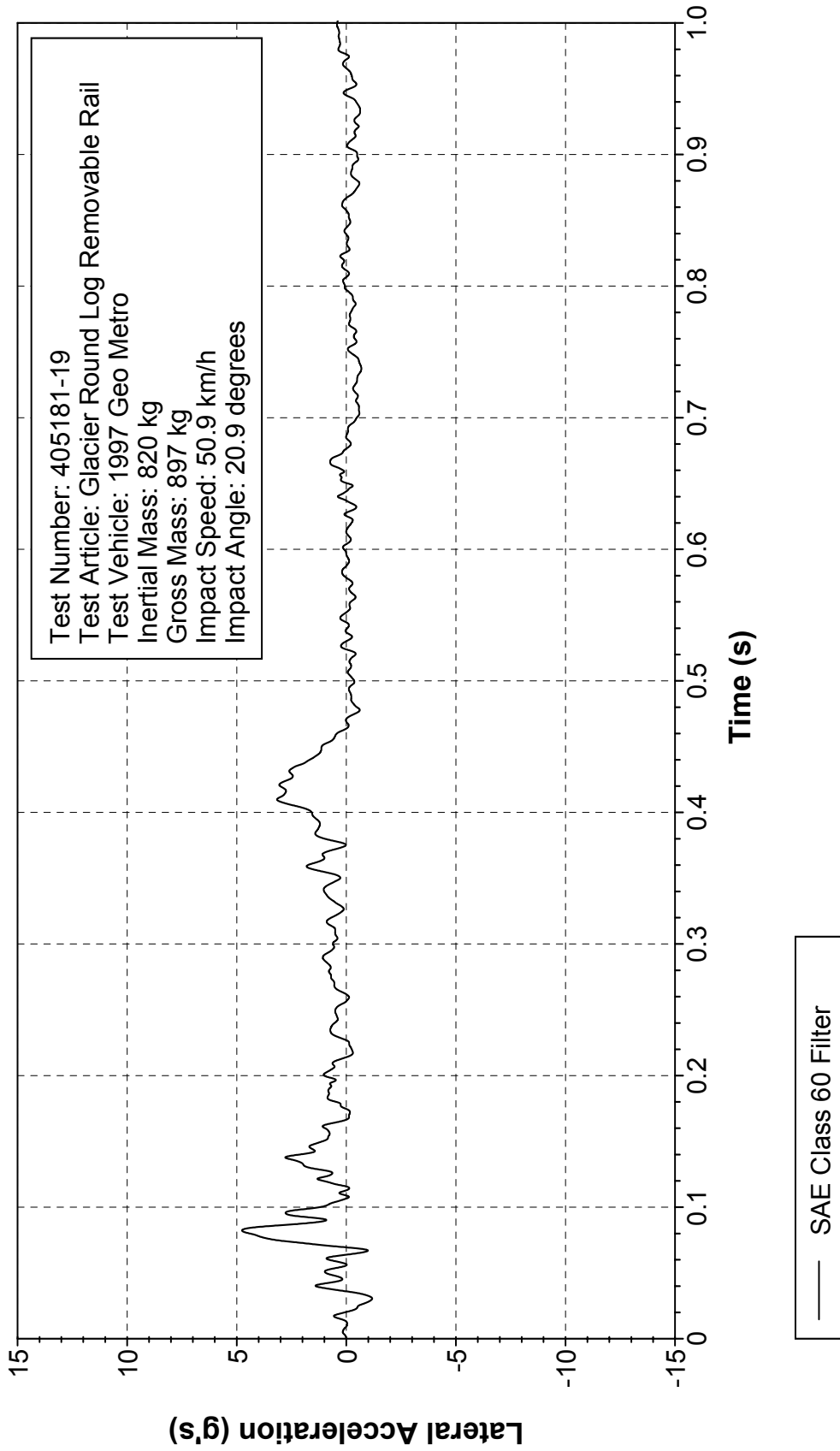
Figure 298. Vehicle lateral accelerometer trace for test 405181-19 (accelerometer located over rear axle).
