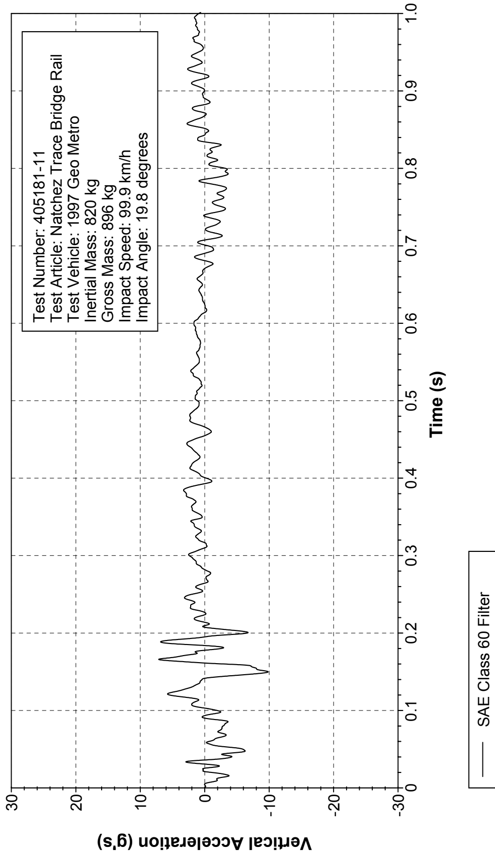
Figure 320. Vehicle vertical accelerometer trace for test 405181-11 (accelerometer located over rear axle).
