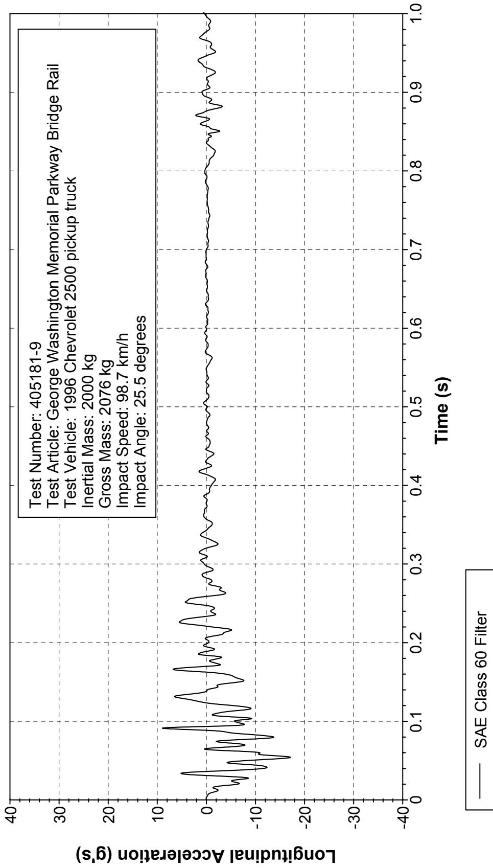
Figure 308. Vehicle longitudinal accelerometer trace for test 405181-9 (accelerometer located at center of gravity).
