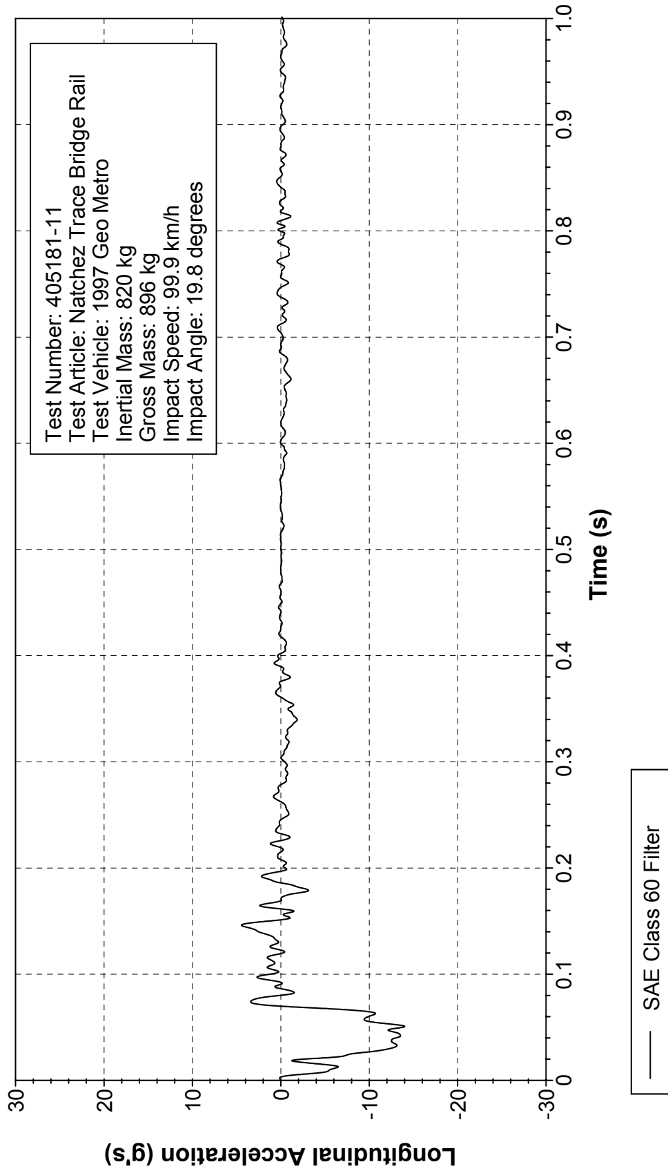
Figure 318. Vehicle longitudinal accelerometer trace for test 405181-11 (accelerometer located over rear axle).
