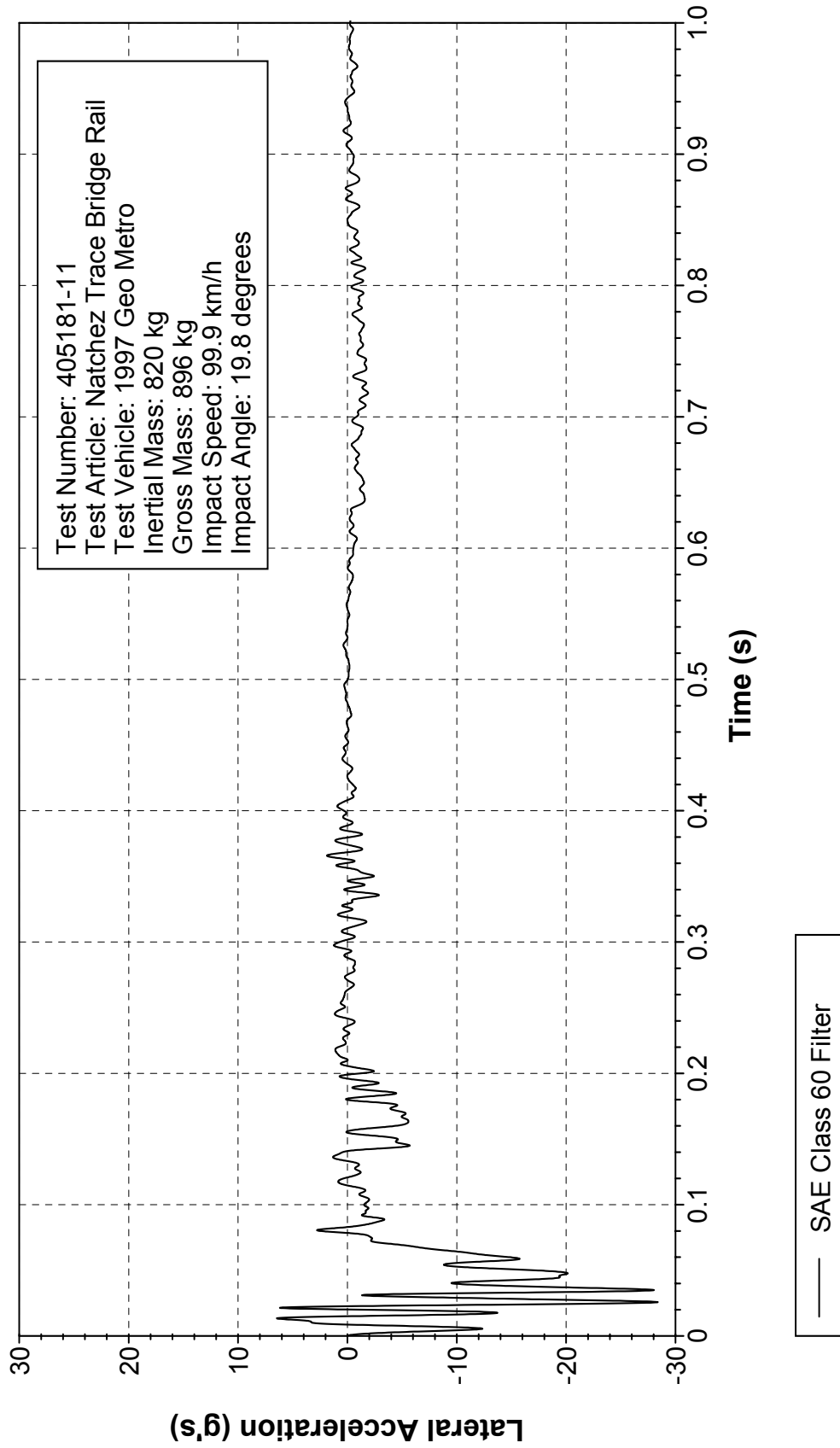
Figure 316. Vehicle lateral accelerometer trace for test 405181-11 (accelerometer located at center of gravity).
