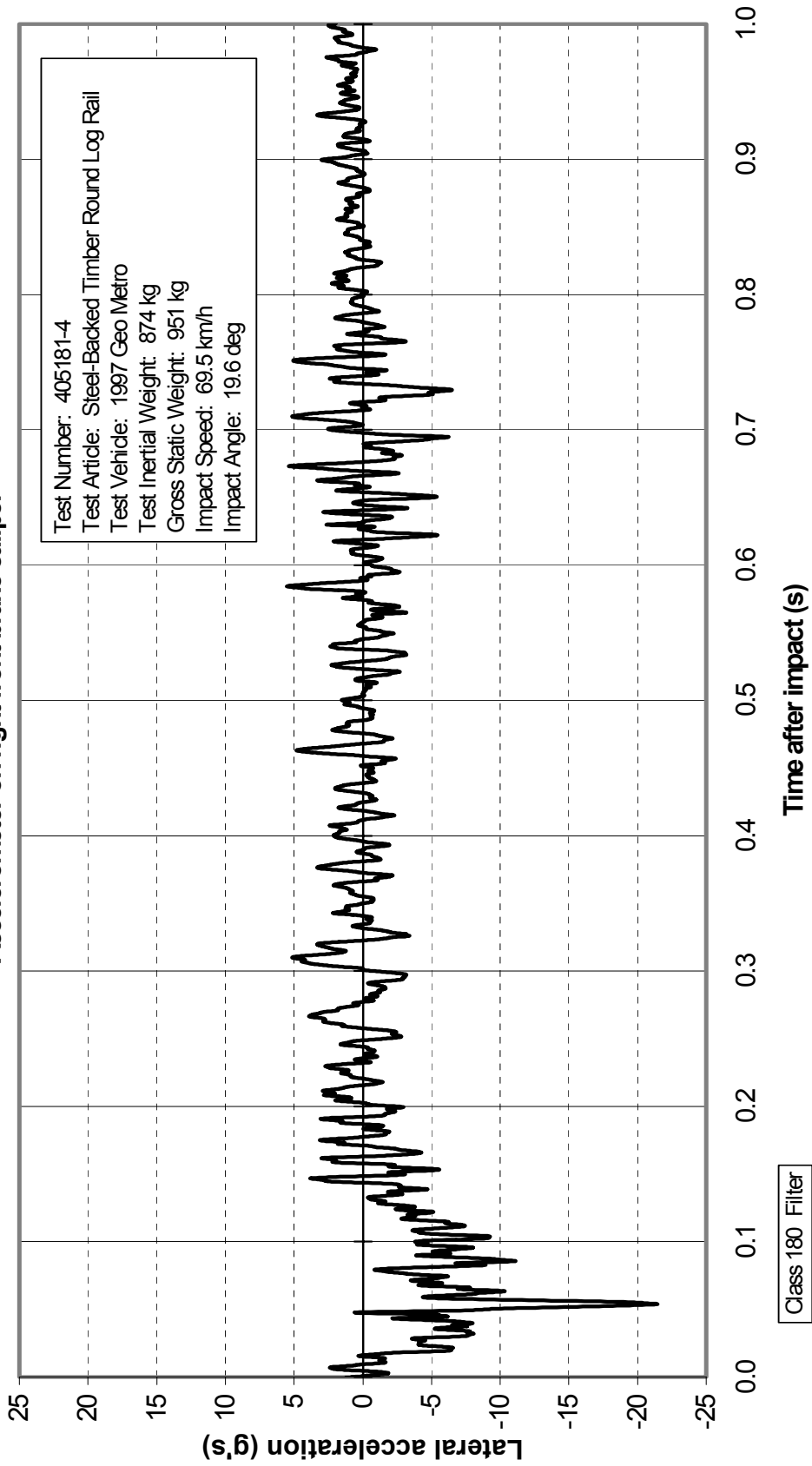
Figure 251. Vehicle lateral accelerometer trace for test 405181-4 (accelerometer located on right front brake caliper).
