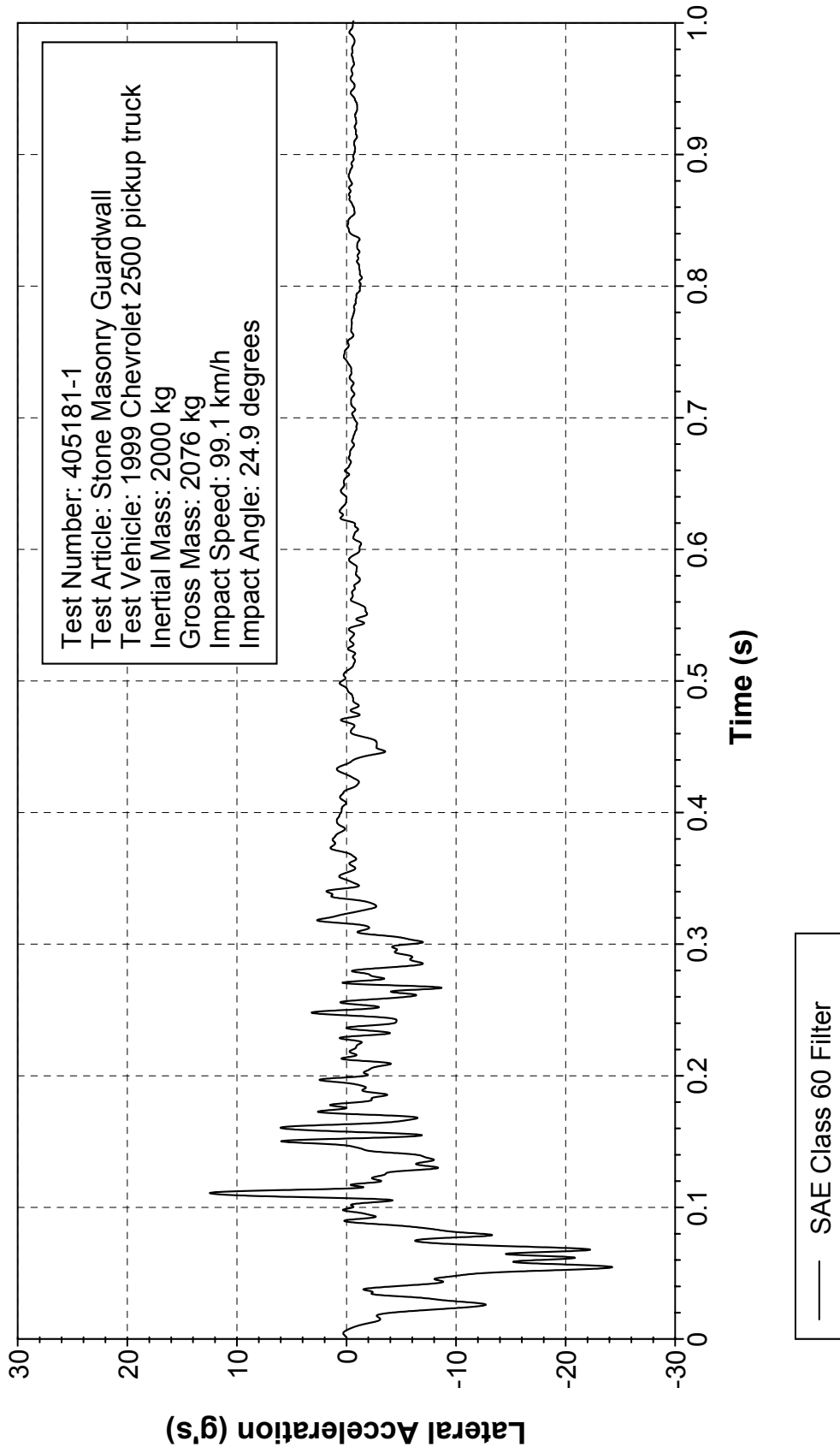
Figure 231. Vehicle lateral accelerometer trace for test 405181-1 (accelerometer located at center of gravity).
