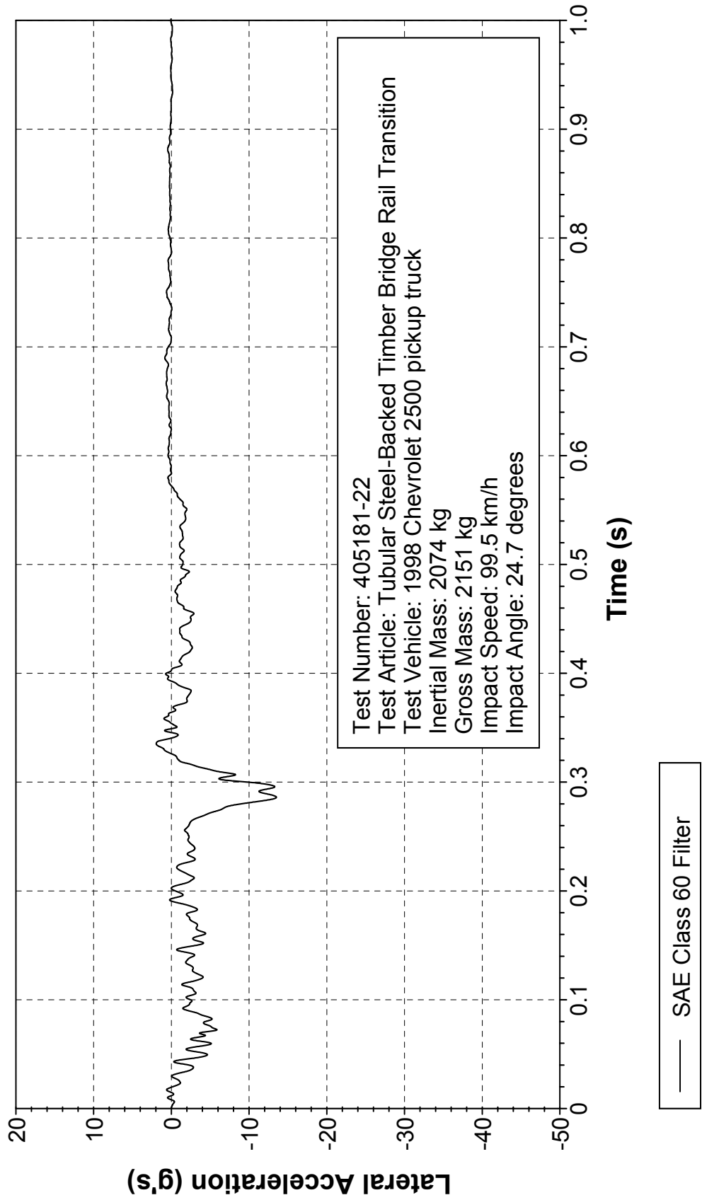
Figure 359. Vehicle lateral accelerometer trace for test 405181-22 (accelerometer located over rear axle).
