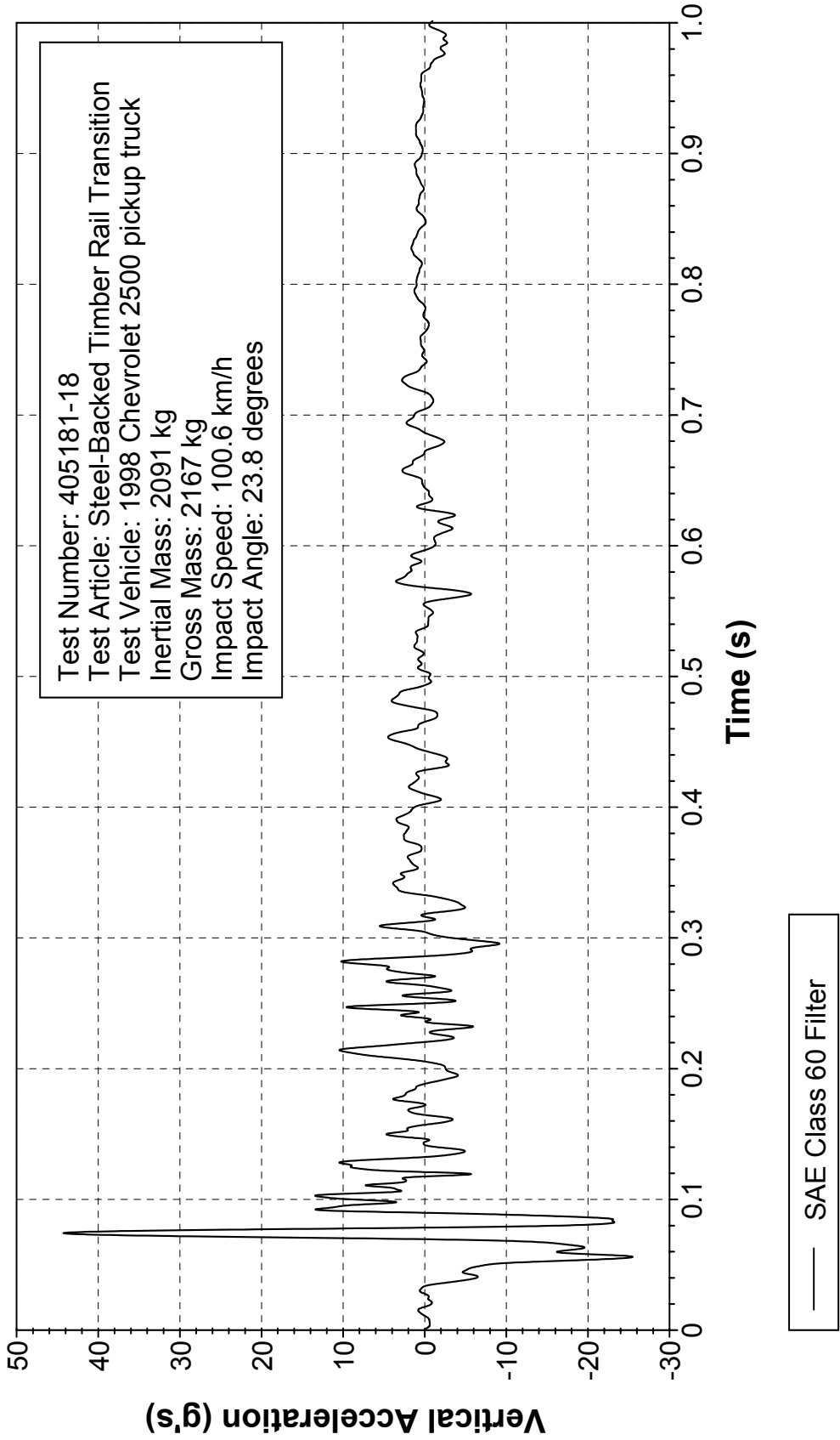
Figure 350. Vehicle vertical accelerometer trace for test 405181-18 (accelerometer located at center of gravity).
