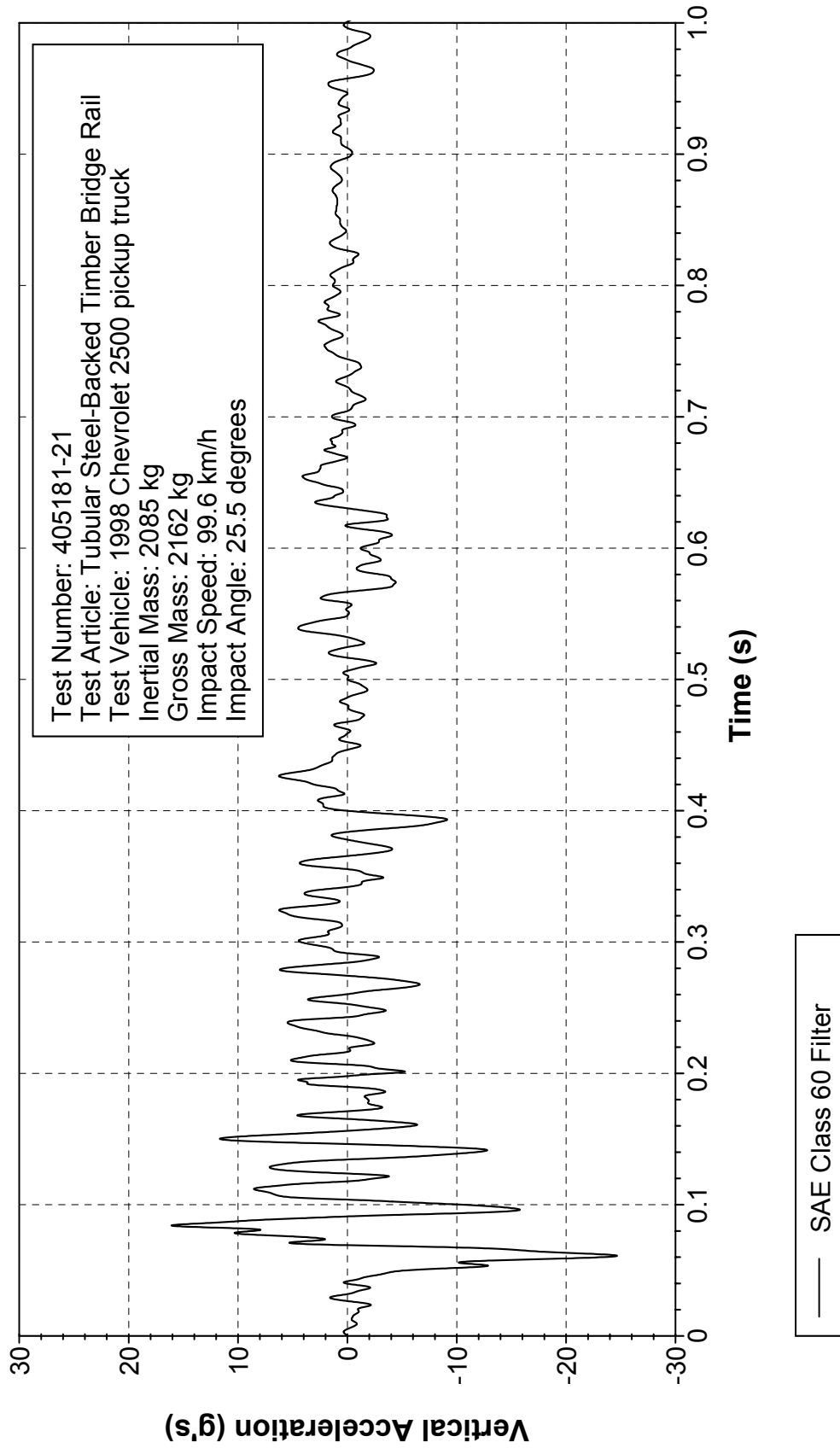
Figure 331. Vehicle vertical accelerometer trace for test 405181-21 (accelerometer located at center of gravity).
