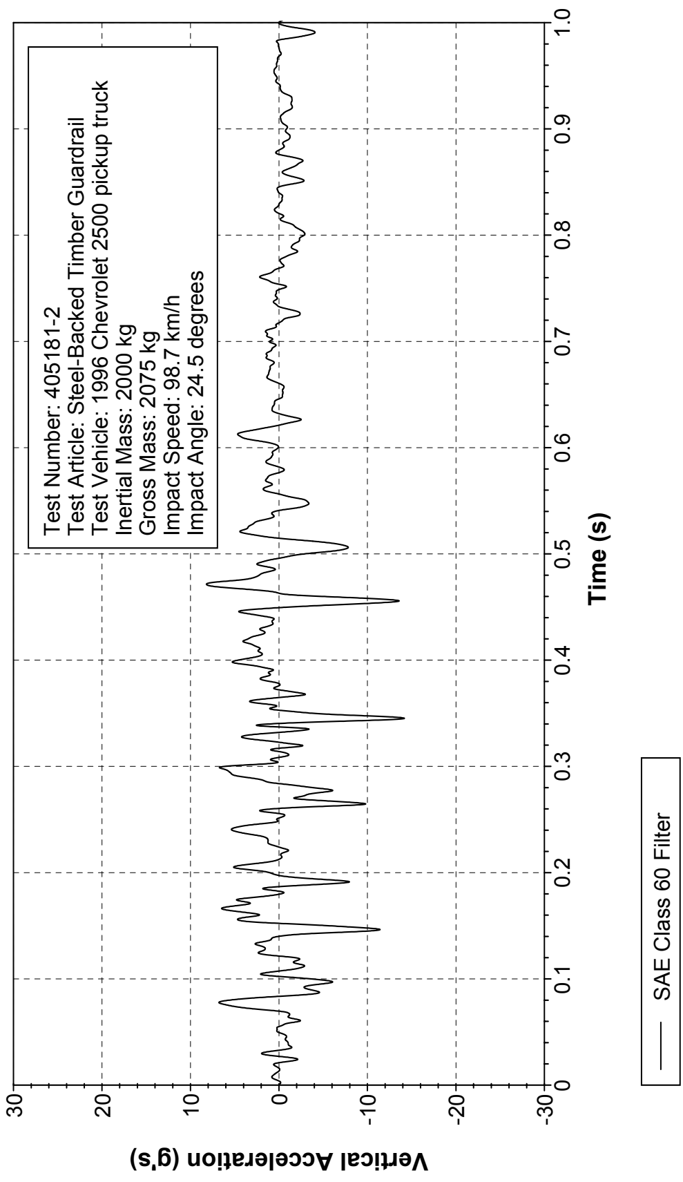
Figure 242. Vehicle vertical accelerometer trace for test 405181-2 (accelerometer located over rear axle).
