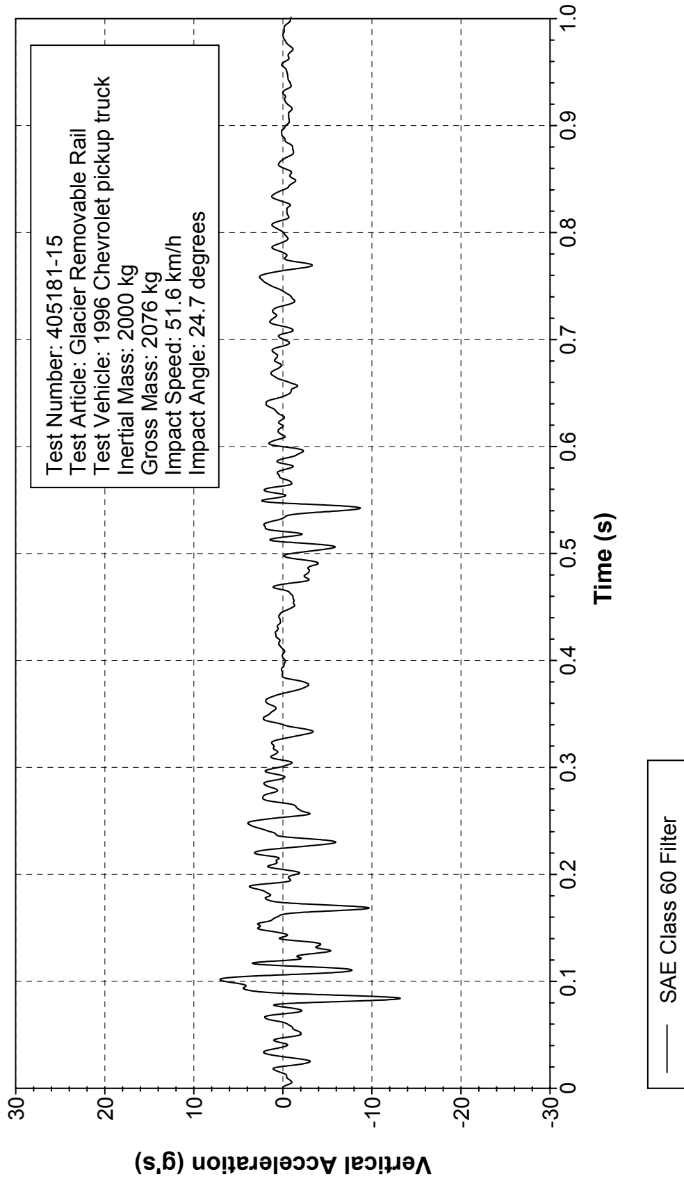
Figure 292. Vehicle vertical accelerometer trace for test 405181-15 (accelerometer located over rear axle).
