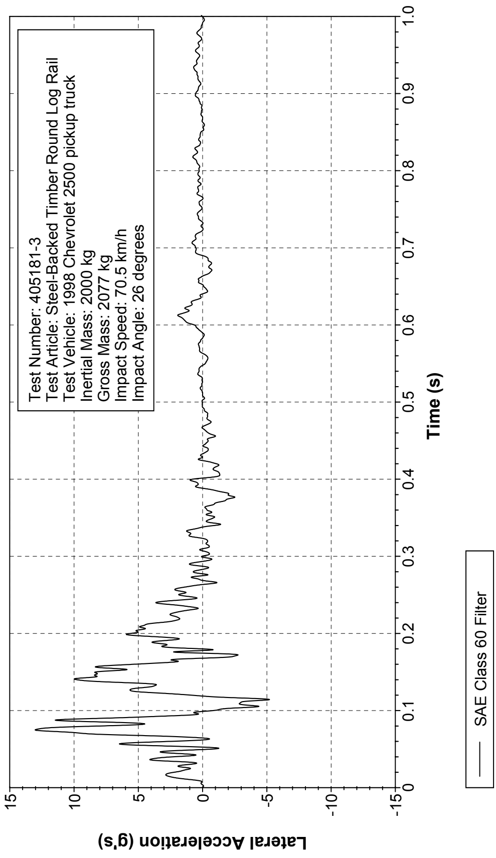
Figure 257. Vehicle lateral accelerometer trace for test 405181-3 (accelerometer located at center of gravity).
