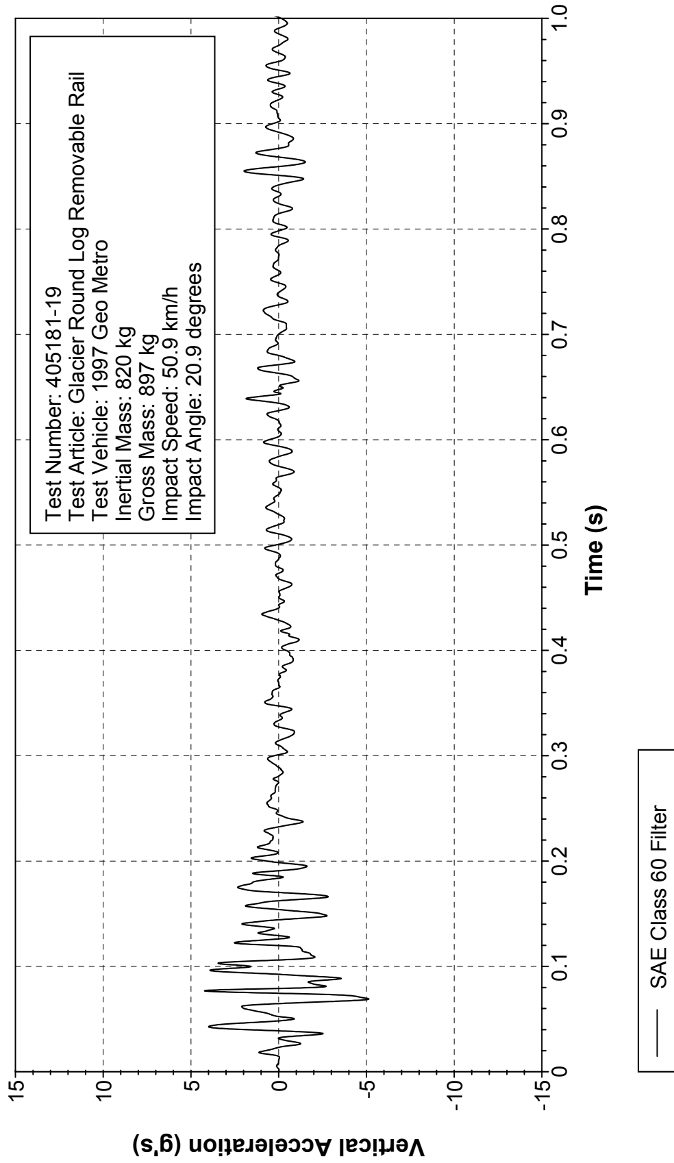
Figure 296. Vehicle vertical accelerometer trace for test 405181-19 (accelerometer located at center of gravity).
