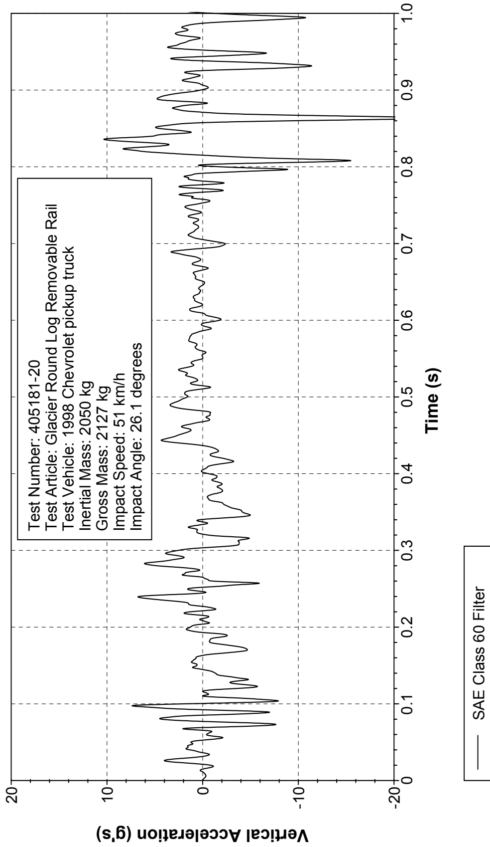
Figure 306. Vehicle vertical accelerometer trace for test 405181-20 (accelerometer located over rear axle).
