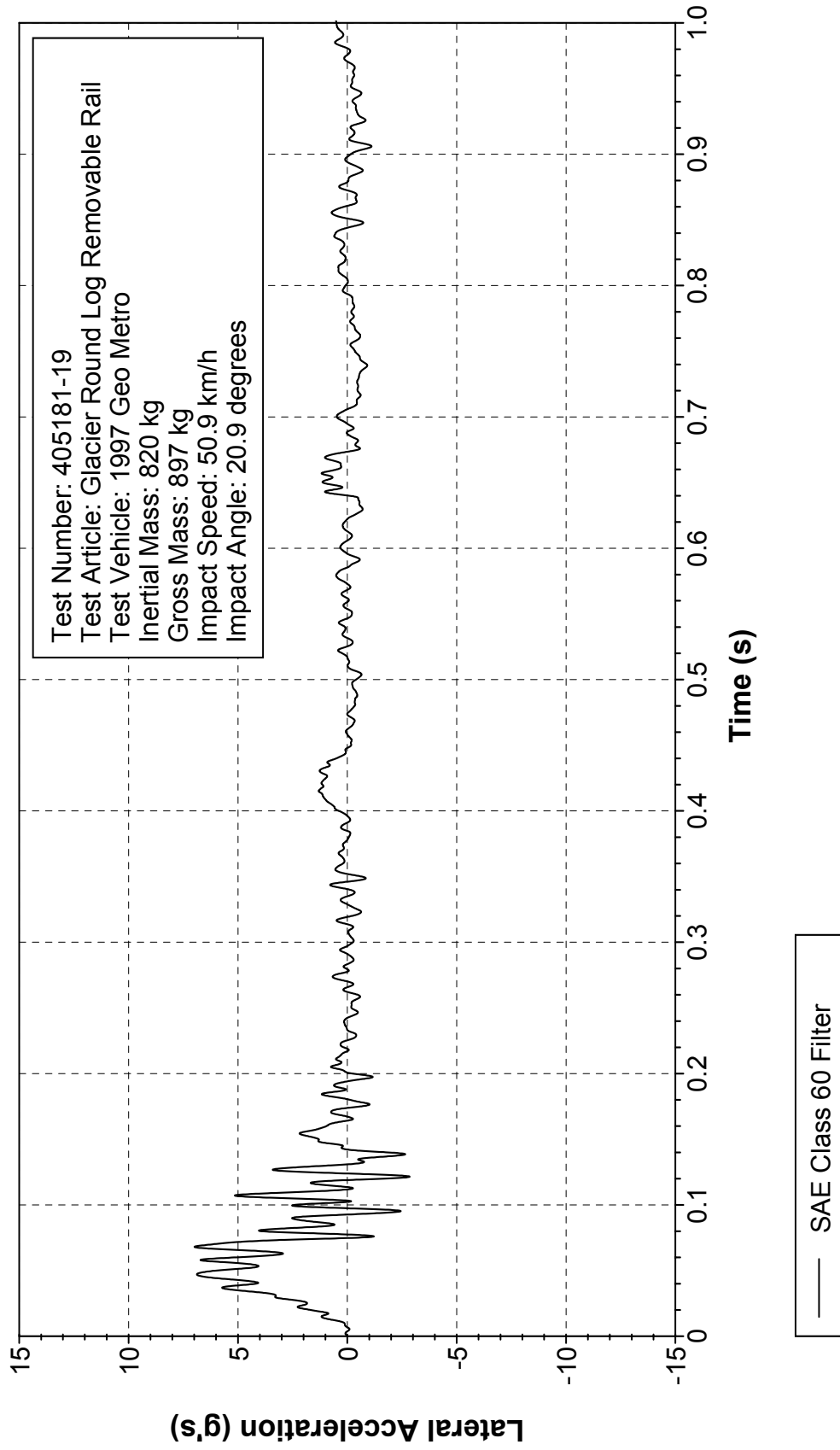
Figure 295. Vehicle lateral accelerometer trace for test 405181-19 (accelerometer located at center of gravity).
