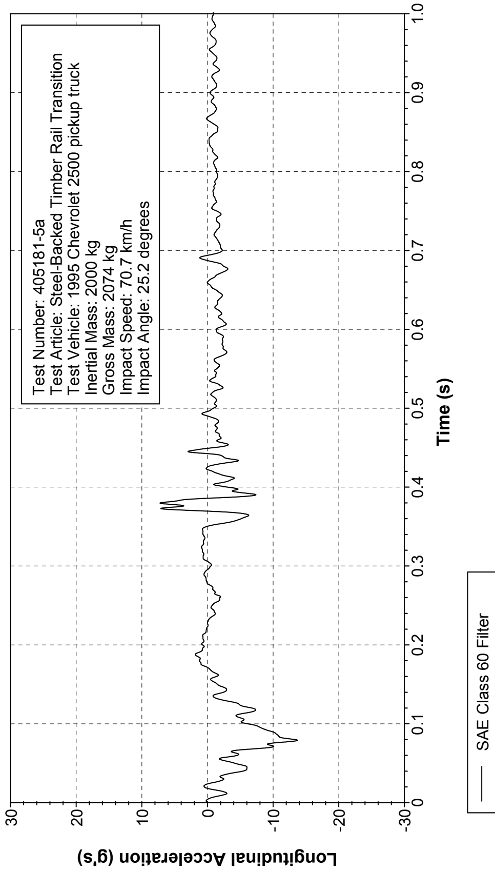
Figure 339. Vehicle longitudinal accelerometer trace for test 405181-5a (accelerometer located over rear axle).
