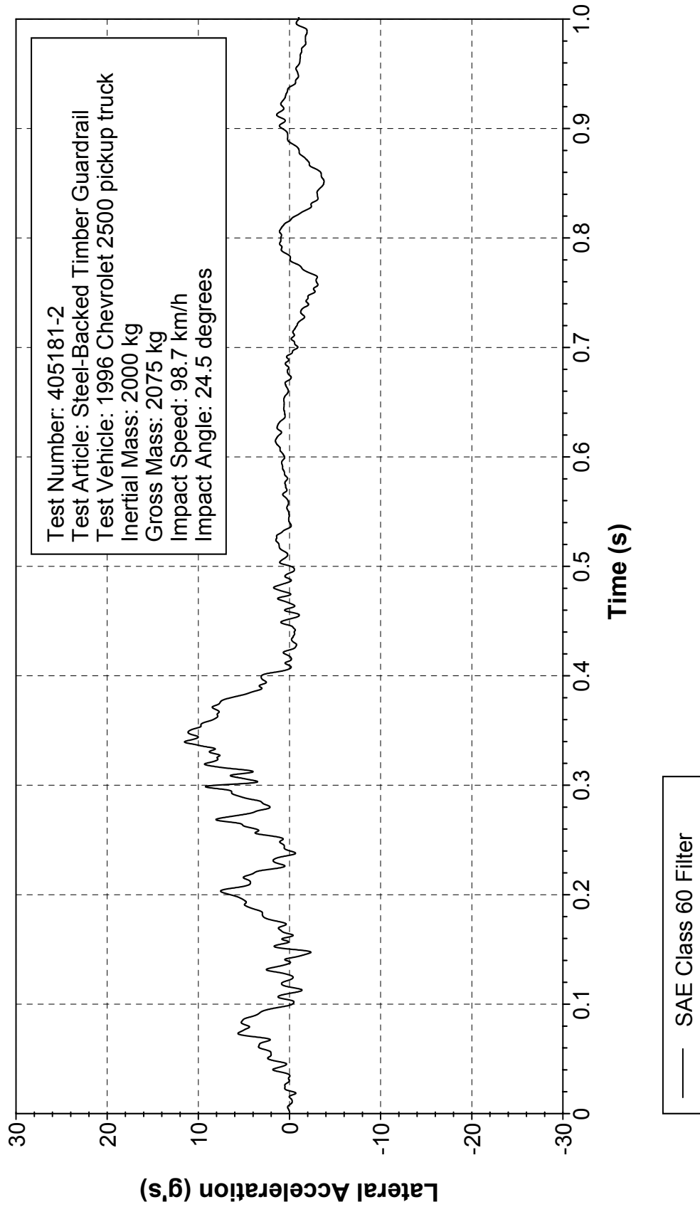
Figure 241. Vehicle lateral accelerometer trace for test 405181-2 (accelerometer located over rear axle).
