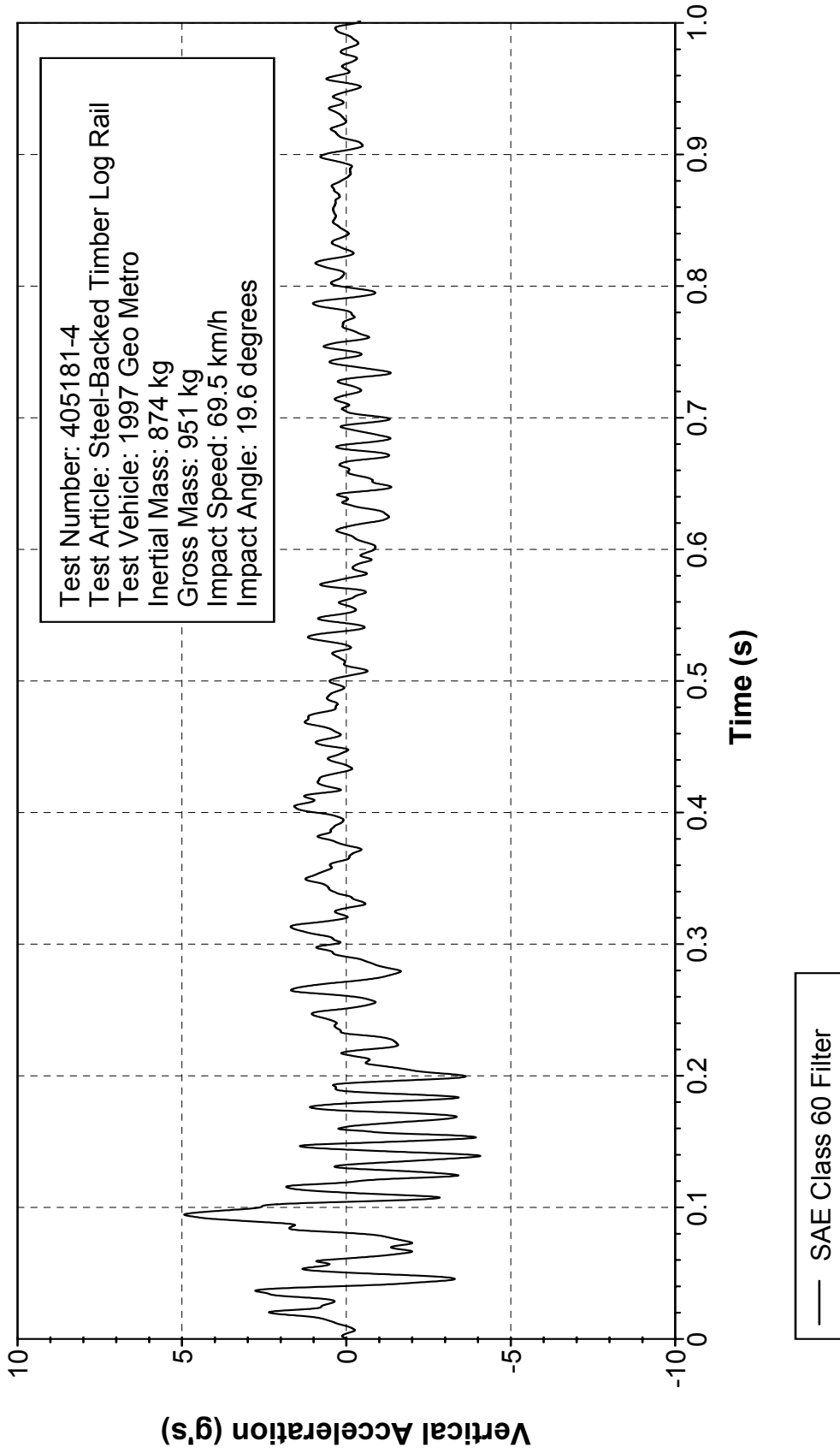
Figure 246. Vehicle vertical accelerometer trace for test 405181-4 (accelerometer located at center of gravity).
