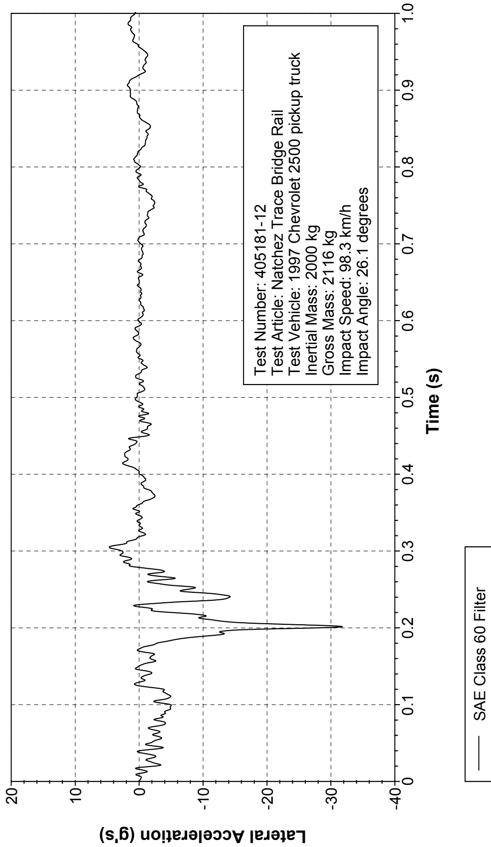
Figure 326. Vehicle lateral accelerometer trace for test 405181-12 (accelerometer located over rear axle).
