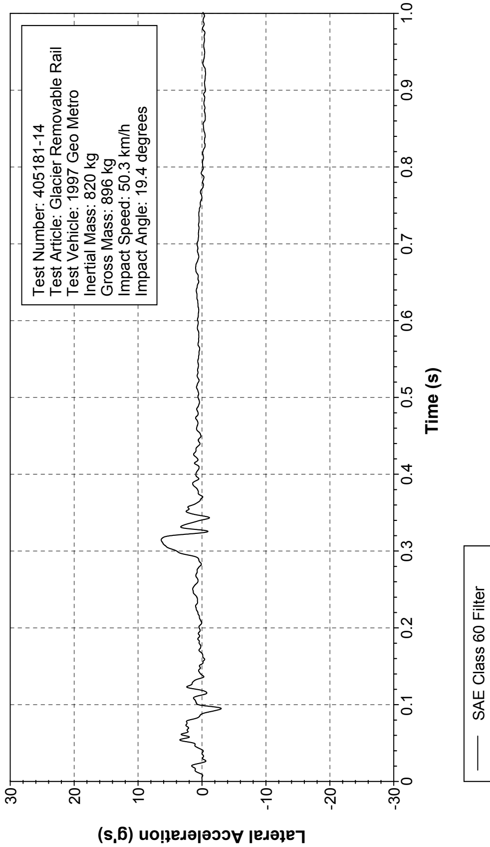
Figure 279. Vehicle lateral accelerometer trace for test 405181-14 (accelerometer located over rear axle).
