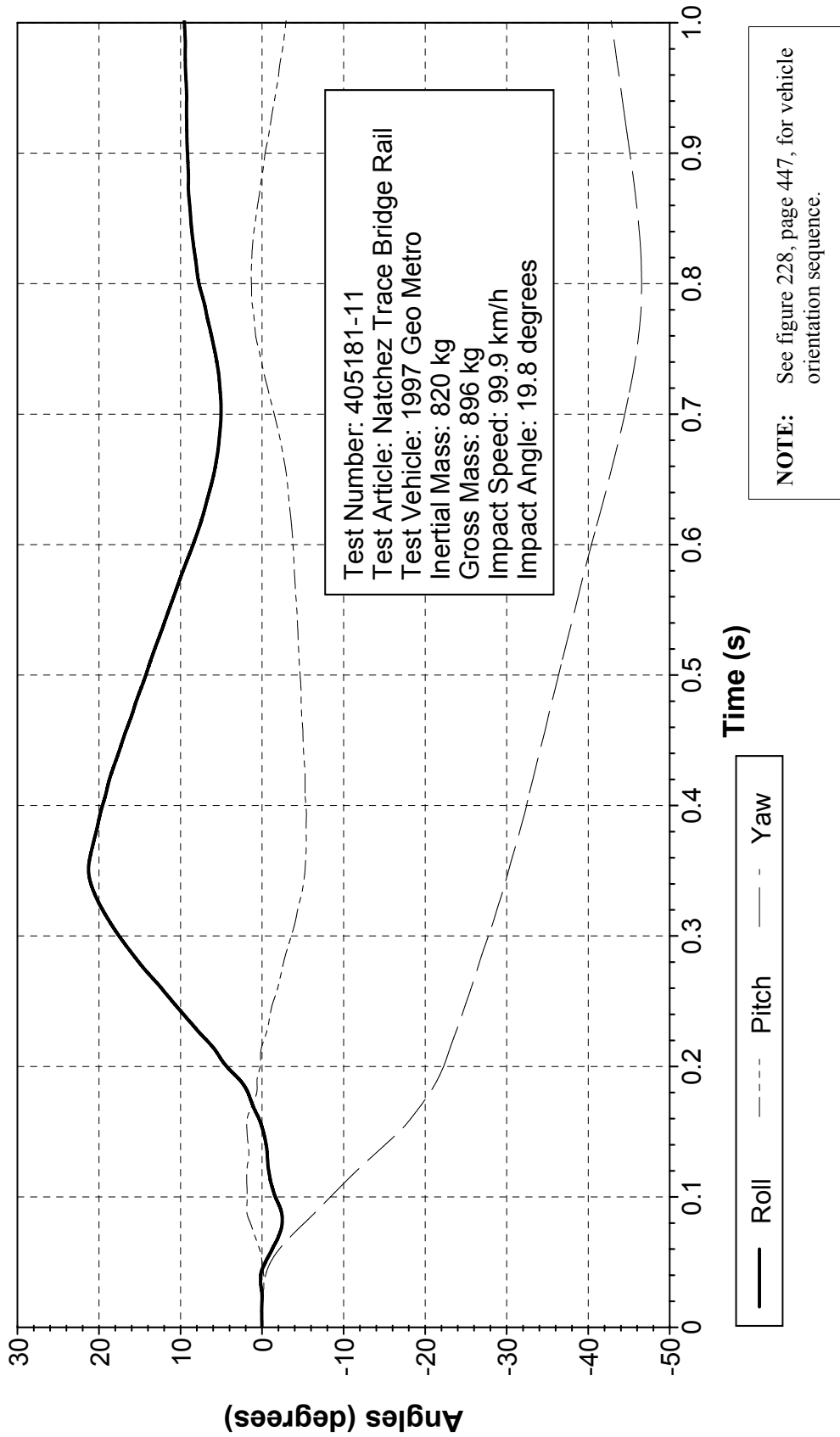
Figure 314. Vehicle angular displacements for test 405181-11.
