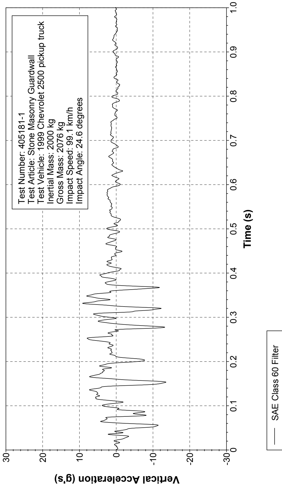
Figure 235. Vehicle vertical accelerometer trace for test 405181-1 (accelerometer located over rear axle).
