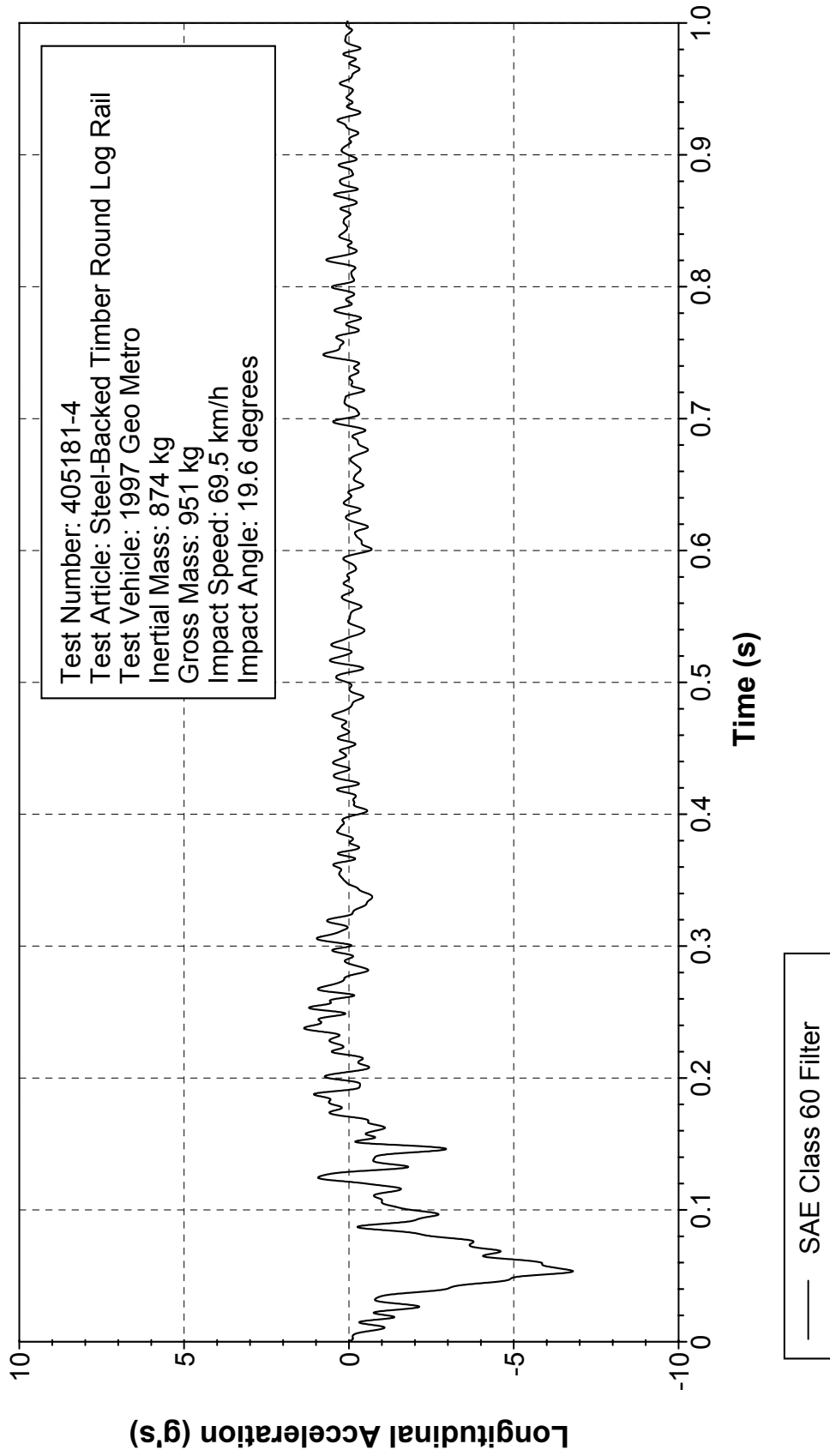
Figure 247. Vehicle longitudinal accelerometer trace for test 405181-4 (accelerometer located over rear axle).
