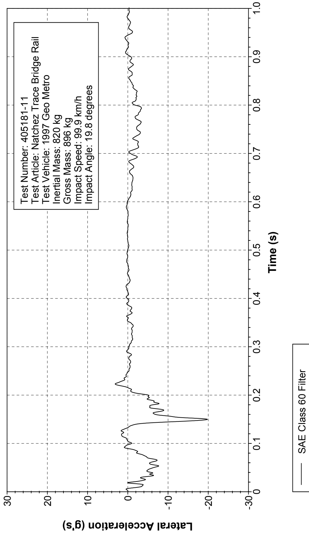
Figure 319. Vehicle lateral accelerometer trace for test 405181-11 (accelerometer located over rear axle).
