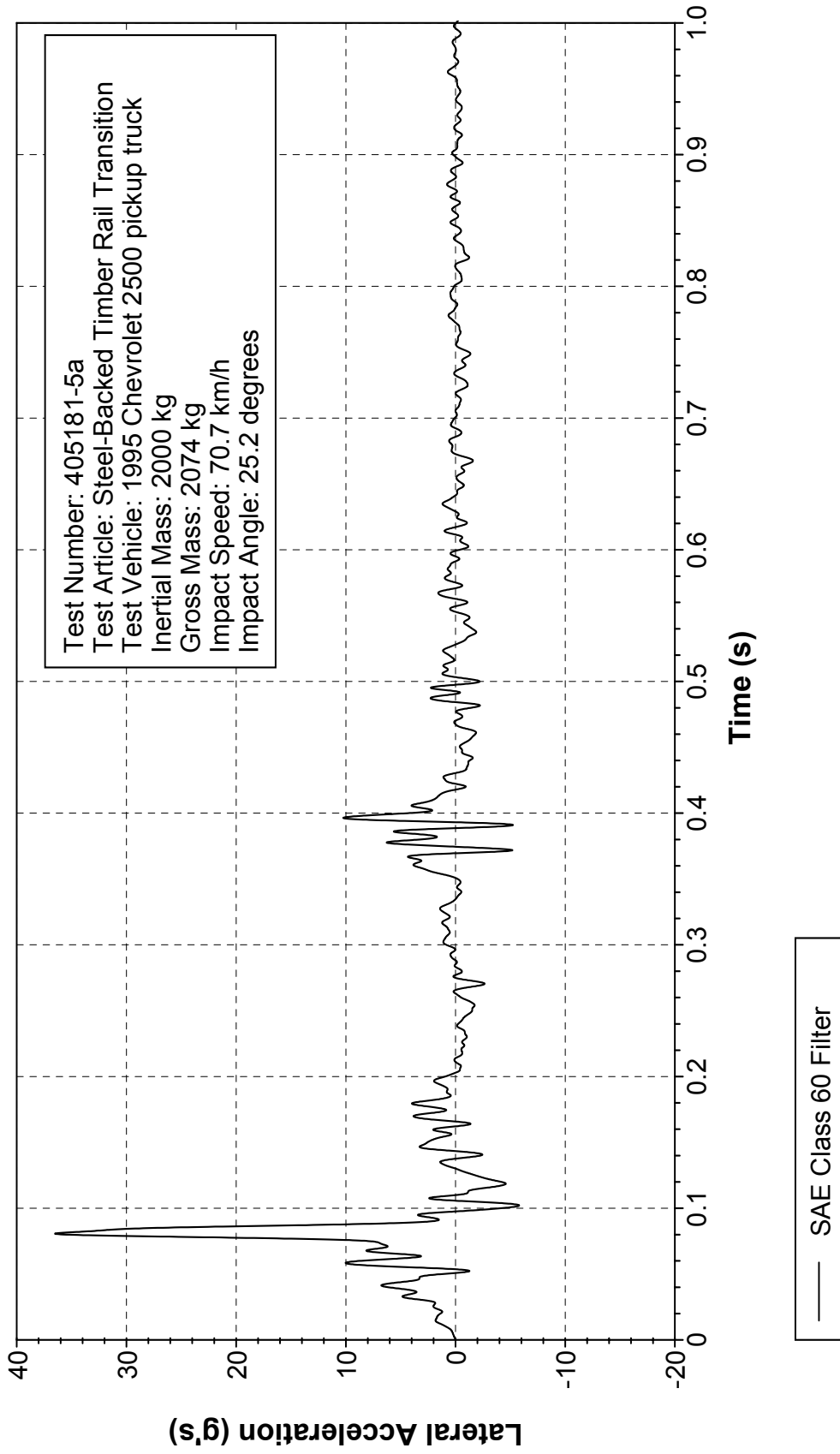
Figure 337. Vehicle lateral accelerometer trace for test 405181-5a (accelerometer located at center of gravity).
