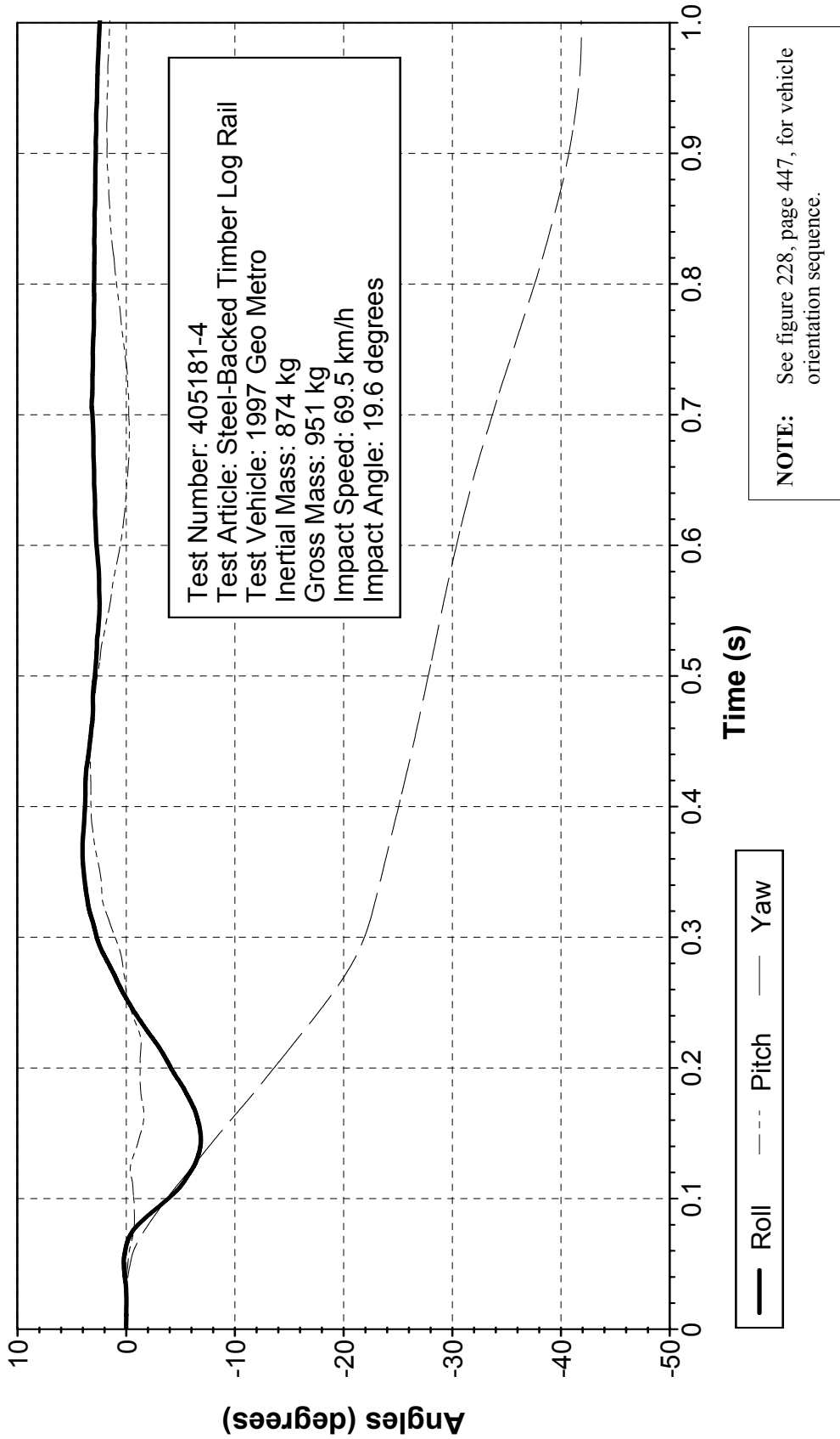
Figure 243. Vehicle angular displacements for test 405181-4.
