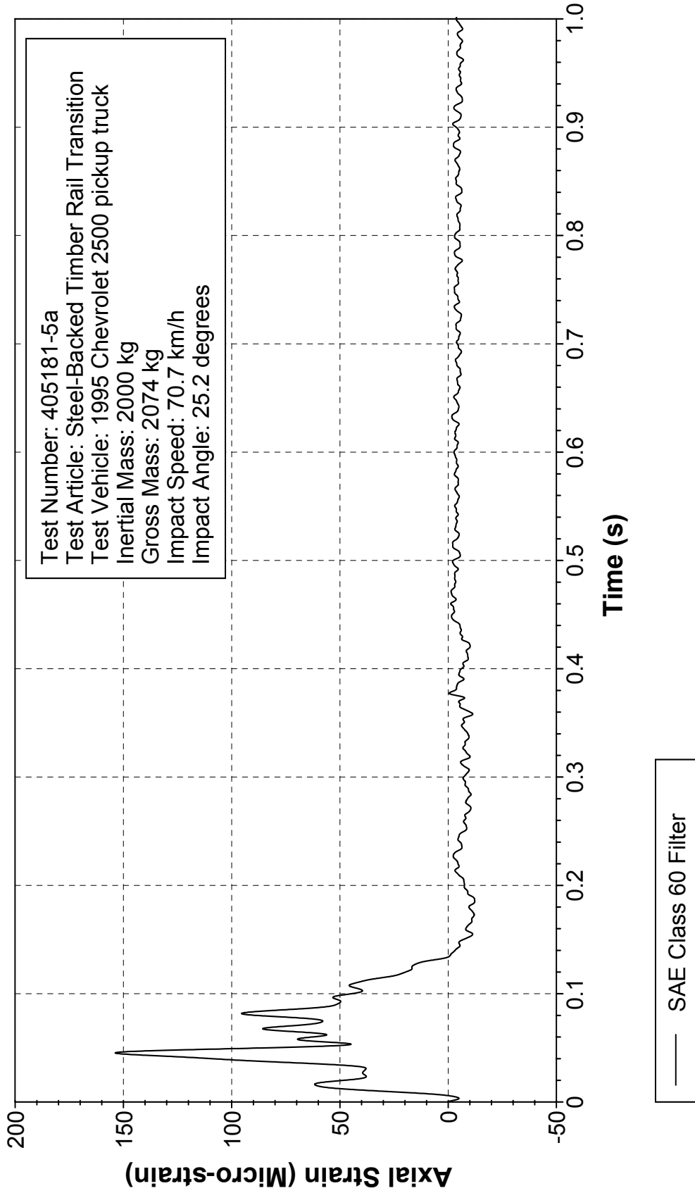
Figure 365. Axial strain, location 4, field side for test 405181-5a.
