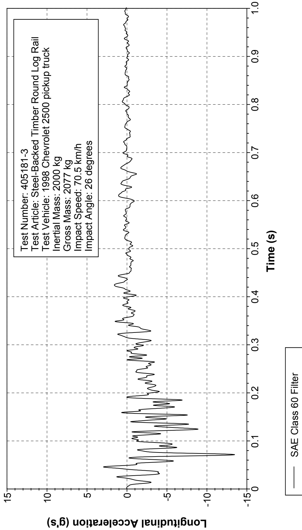
Figure 256. Vehicle longitudinal accelerometer trace for test 405181-3 (accelerometer located at center of gravity).
