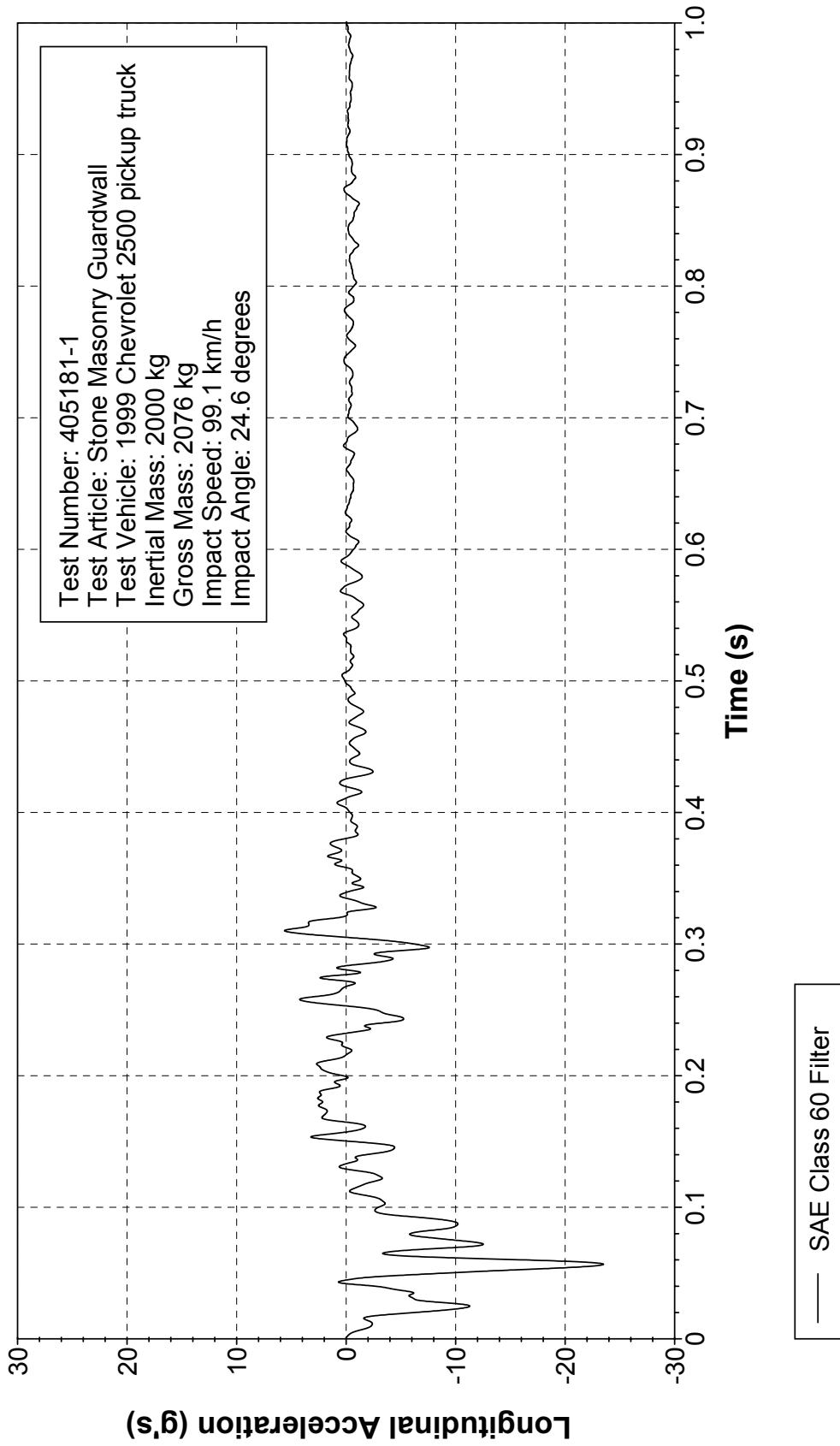
Figure 233. Vehicle longitudinal accelerometer trace for test 405181-1 (accelerometer located over rear axle).
