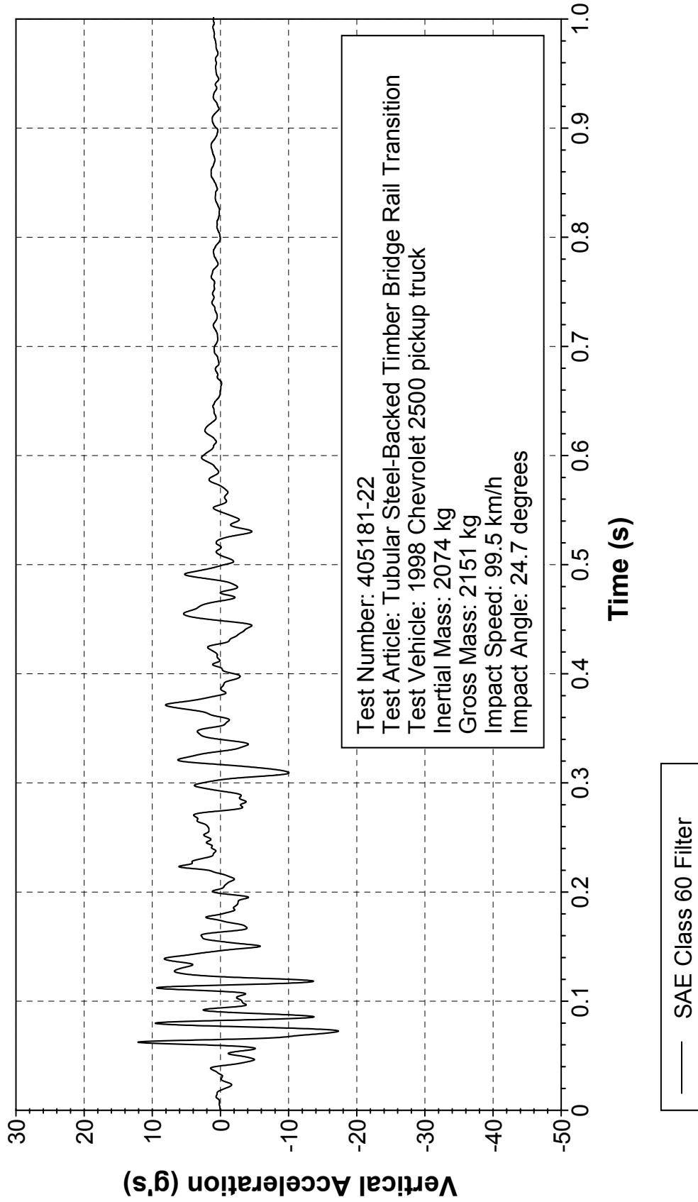
Figure 357. Vehicle vertical accelerometer trace for test 405181-22 (accelerometer located at center of gravity).
