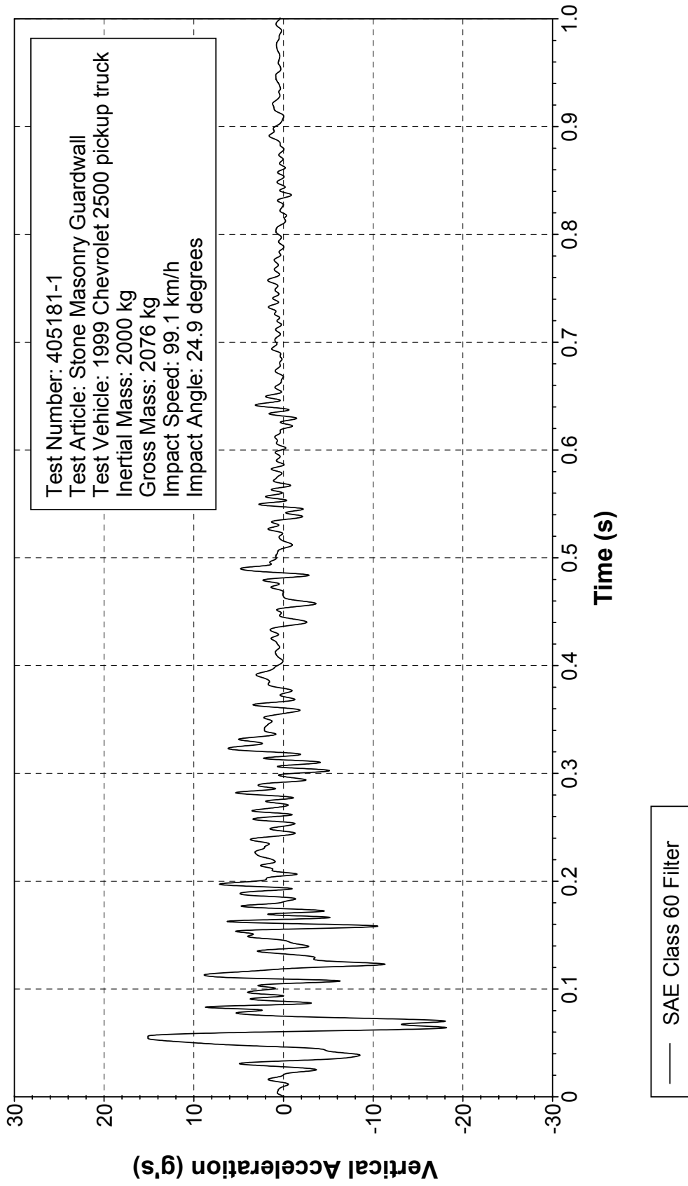
Figure 232. Vehicle vertical accelerometer trace for test 405181-1 (accelerometer located at center of gravity).
