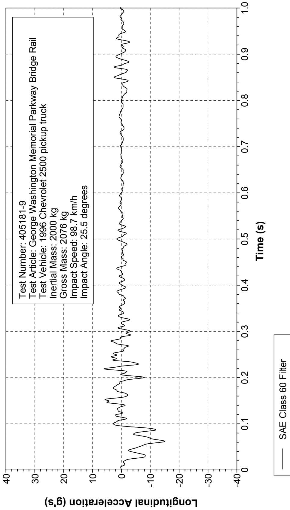
Figure 311. Vehicle longitudinal accelerometer trace for test 405181-9 (accelerometer located over rear axle).
