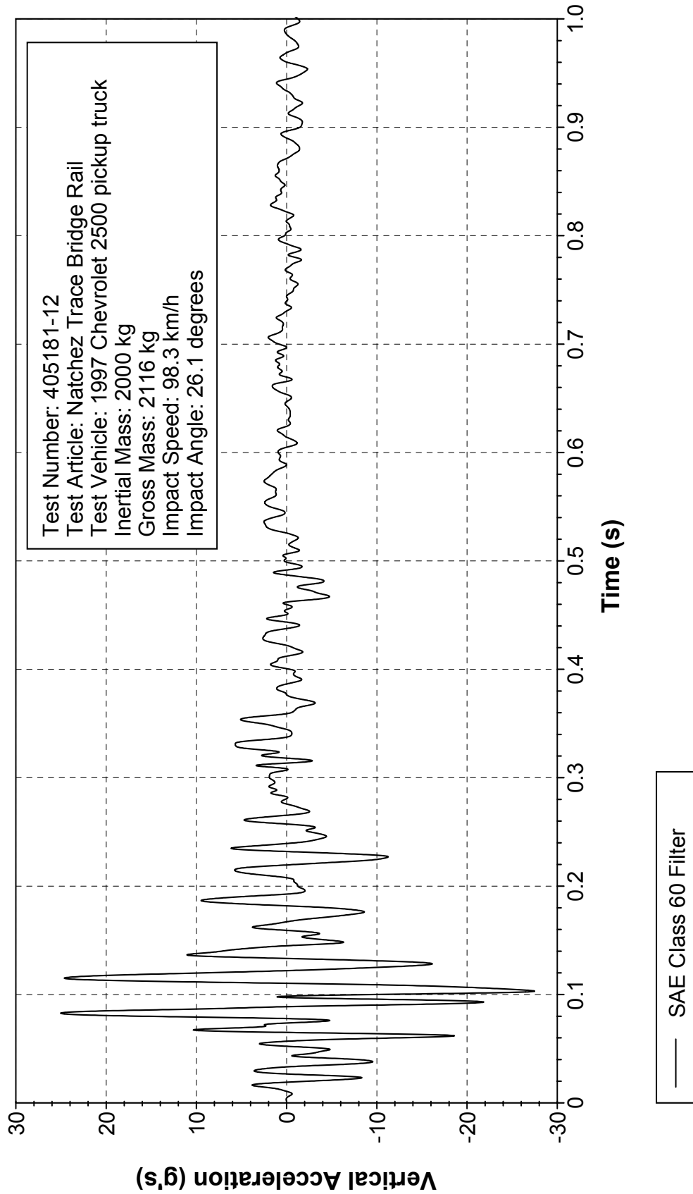
Figure 324. Vehicle vertical accelerometer trace for test 405181-12 (accelerometer located at center of gravity).
