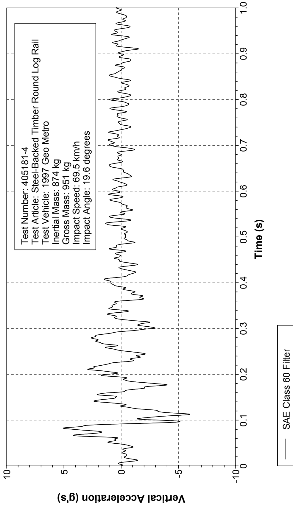
Figure 249. Vehicle vertical accelerometer trace for test 405181-4 (accelerometer located over rear axle).
