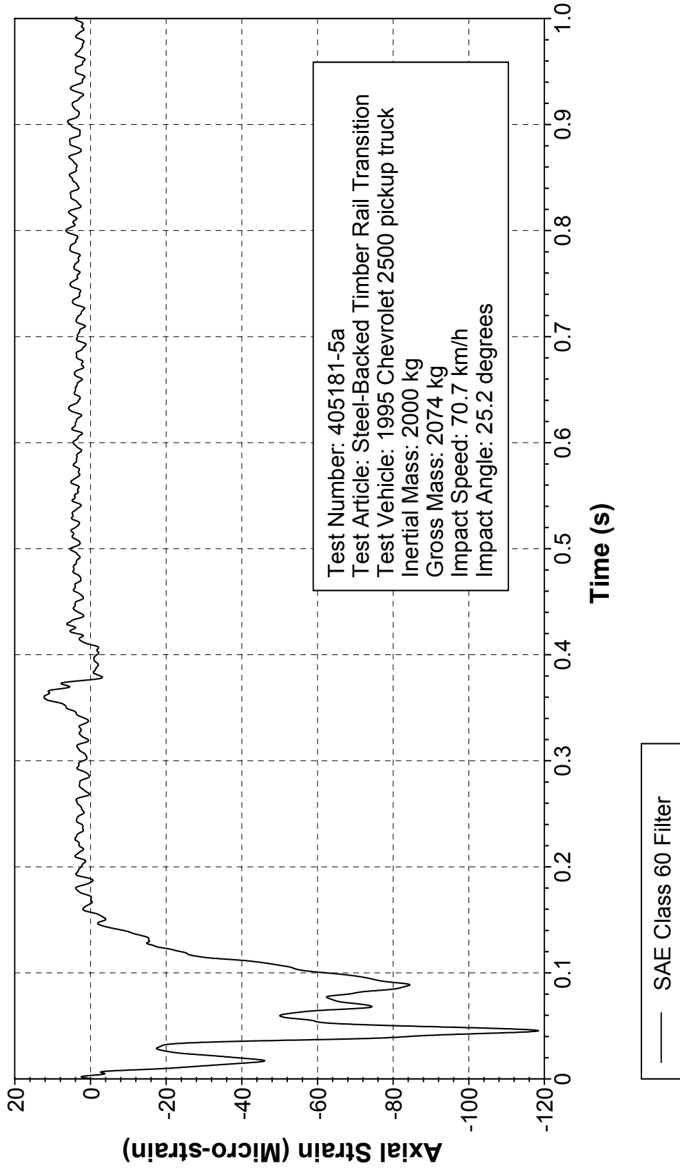
Figure 366. Axial strain, location 5, field side for test 405181-5a.
