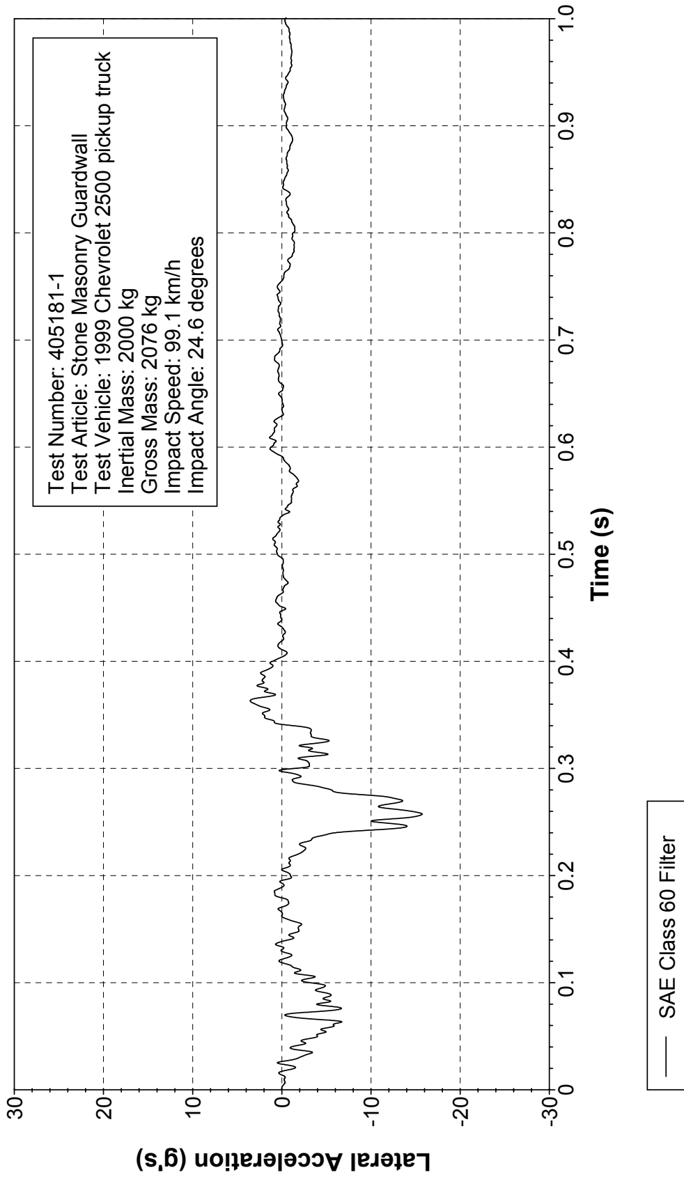
Figure 234. Vehicle lateral accelerometer trace for test 405181-1 (accelerometer located over rear axle).
