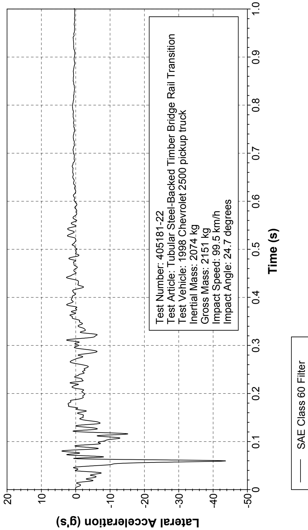
Figure 356. Vehicle lateral accelerometer trace for test 405181-22 (accelerometer located at center of gravity).
