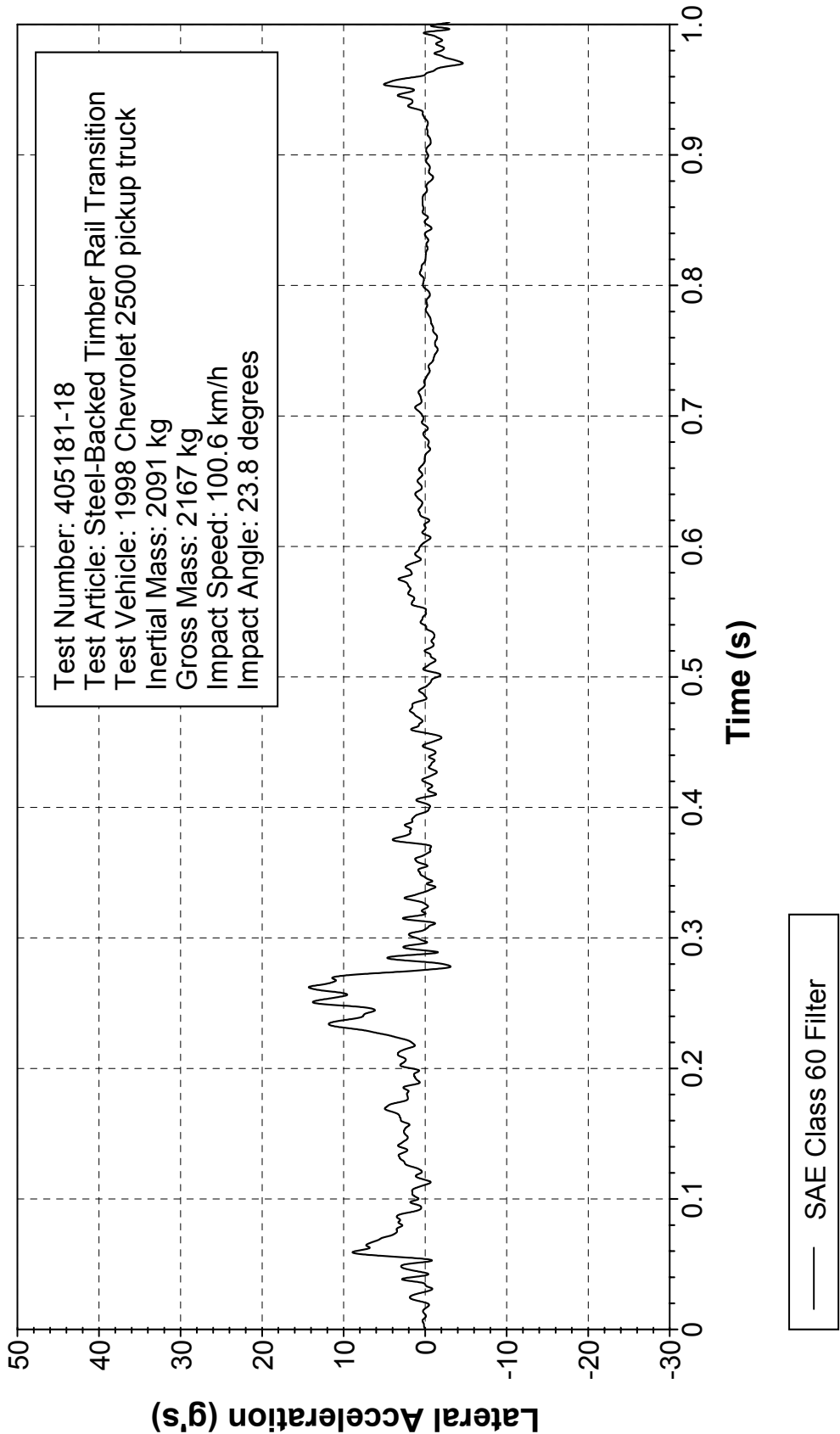
Figure 352. Vehicle lateral accelerometer trace for test 405181-18 (accelerometer located over rear axle).
